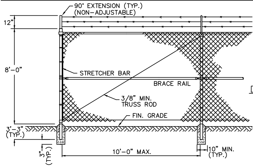
DETAIL TYPICAL FENCE CORNER
