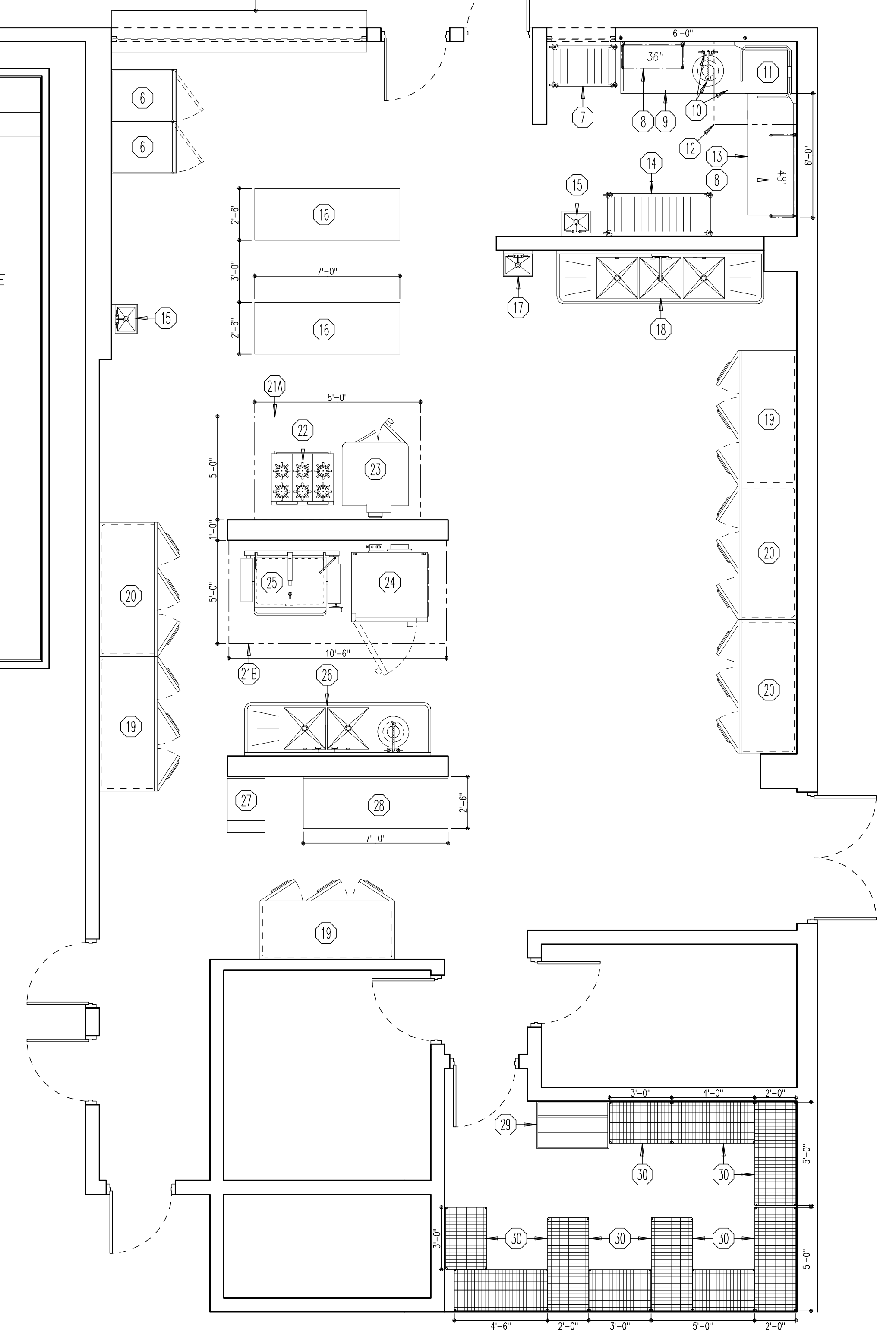
SCHEMATIC PLAN
