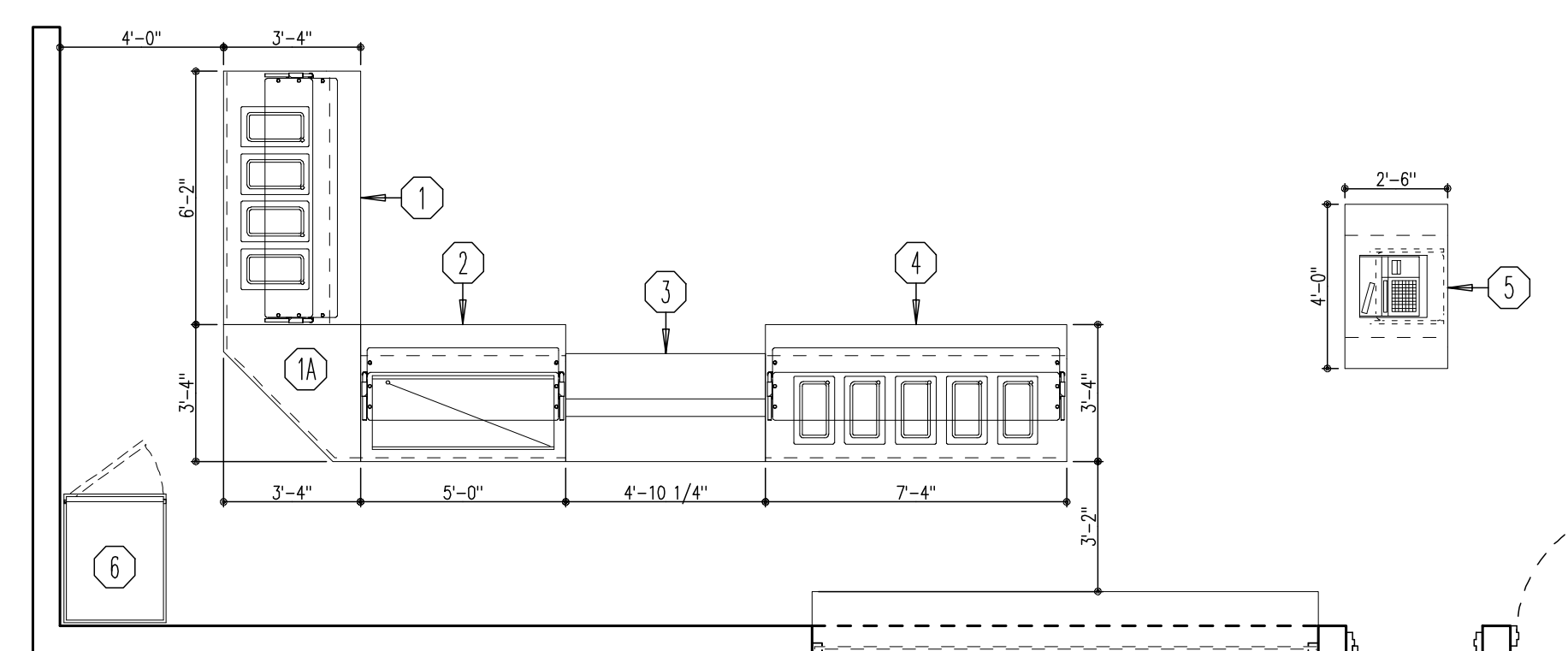
SCHEMATIC PLAN
