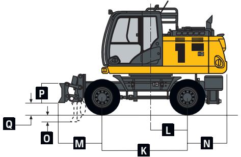
190G W EXCAVATOR WITH FRONT BLADE AND REAR OUTRIGGER
