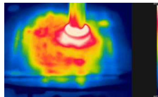
Thermogram T-05
