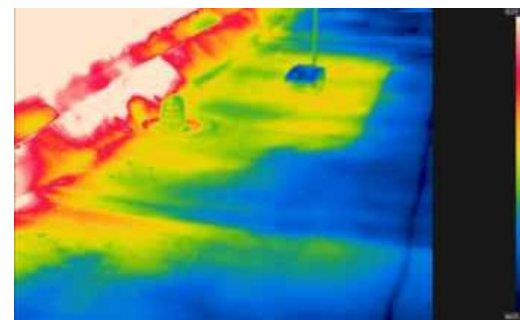
Thermogram T-04
