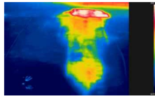
Thermogram T-01
