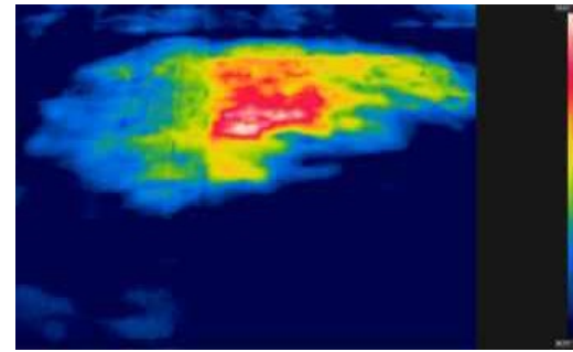
Thermogram T-01
