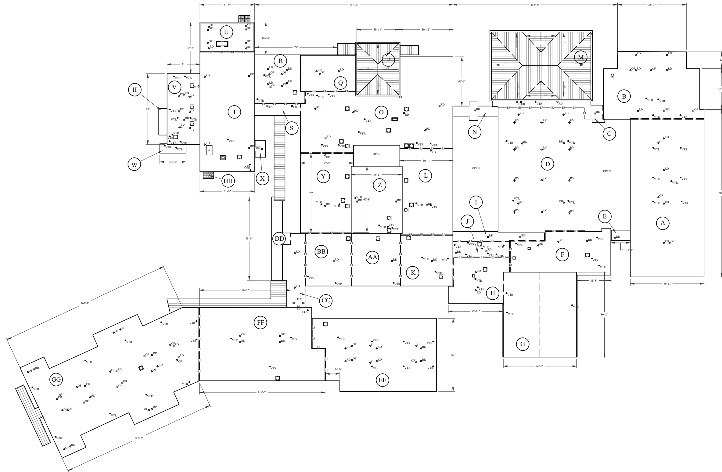
JESSE BOYD ELEMENTARY OVERALL ROOF PLAN
