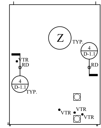
ROOF AREA Z
