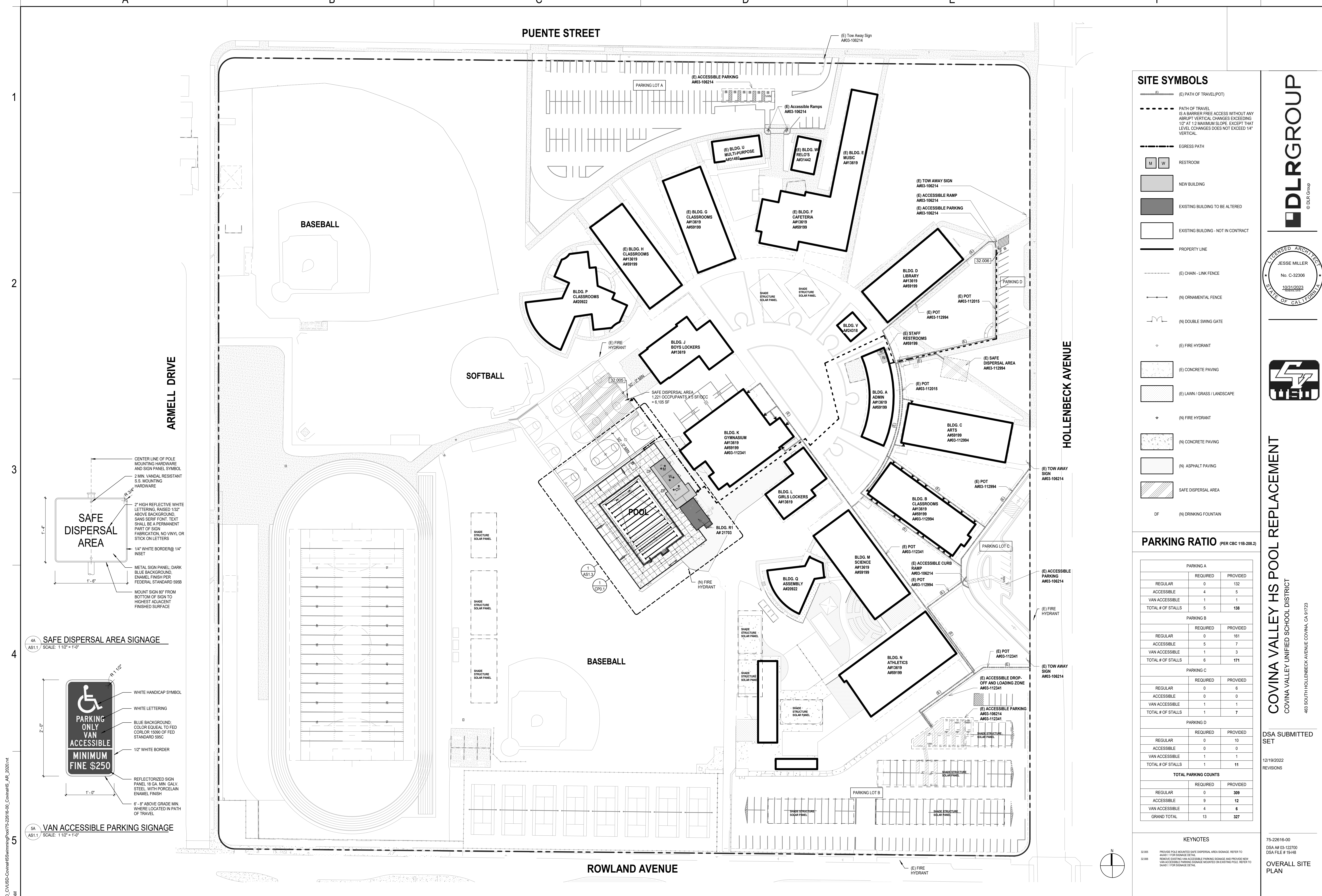
REMODEL SITE PLAN SCALE: 1" = 50'-0"
