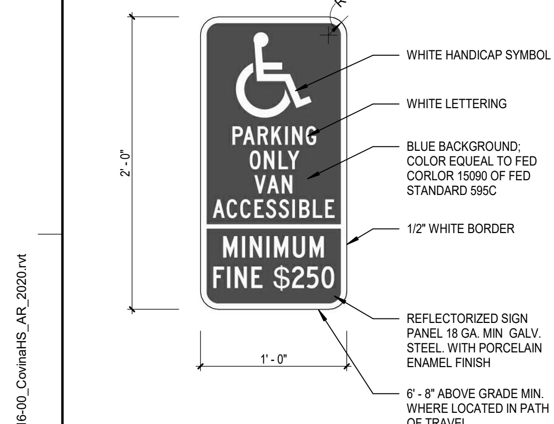
5A VAN ACCESSIBLE PARKING SIGNAGE AS1.1 SCALE: 1/12" = 1'-0"
