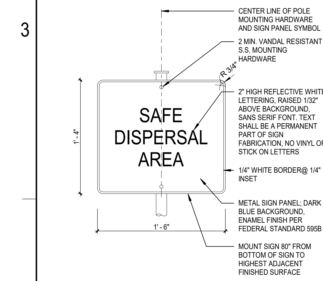
4A SAFE DISPERSAL AREA SIGNAGE AS1.1 SCALE: 1/12" = 1'-0"
