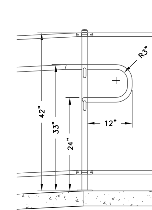
TYPICAL GRAB BAR DETAIL N.T.S.
