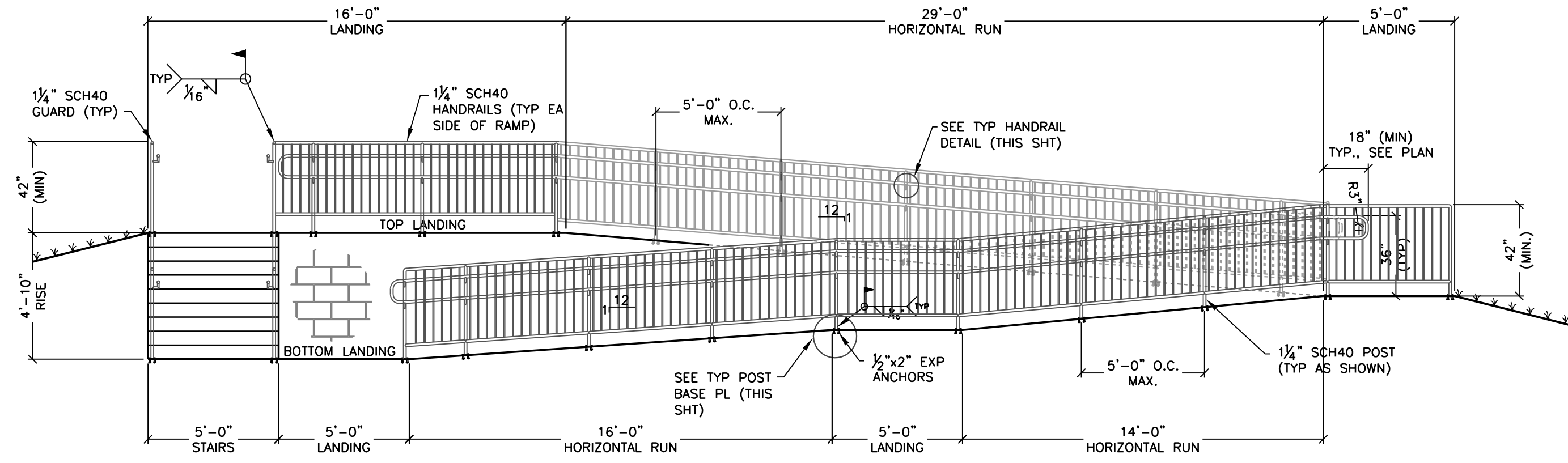
RAMP FRONT ELEVATION SCALE: 1"=5'-0"
