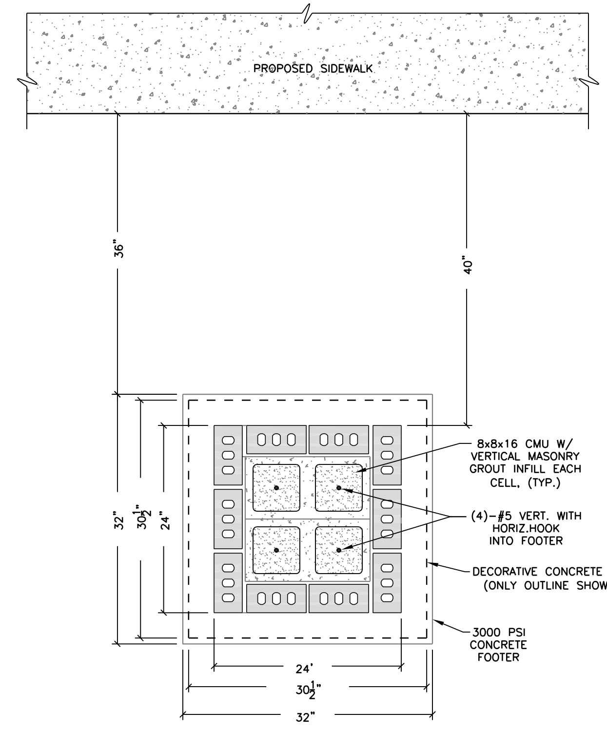
COLUMN PLAN VIEW SCALE: 1"=1'-0"
