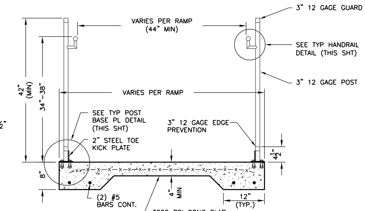
TYPICAL RAMP SECTION DETAIL SCALE: 3/4"=1'-0"
