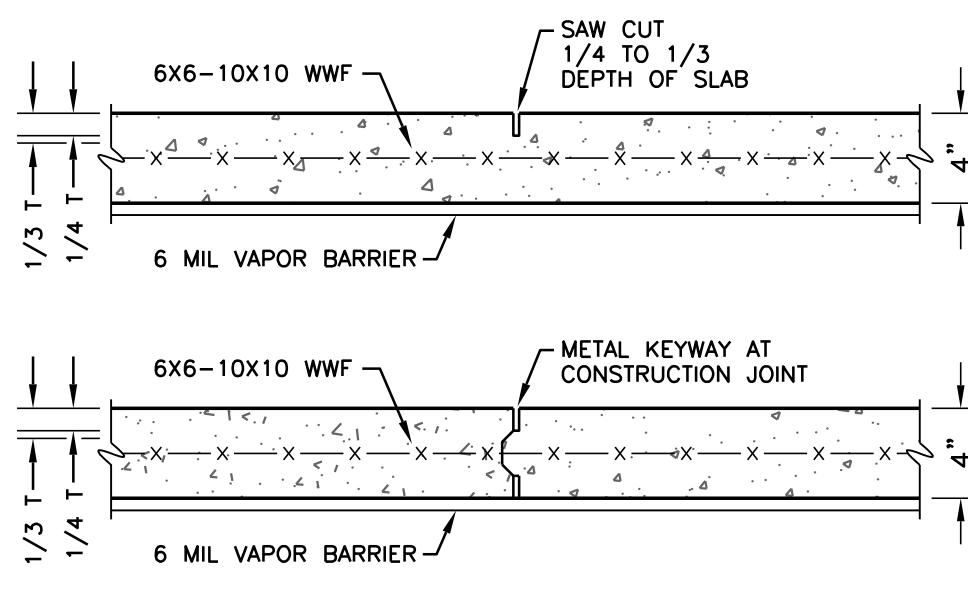
TYPICAL SLAB JOINT DETAILS NOT TO SCALE
