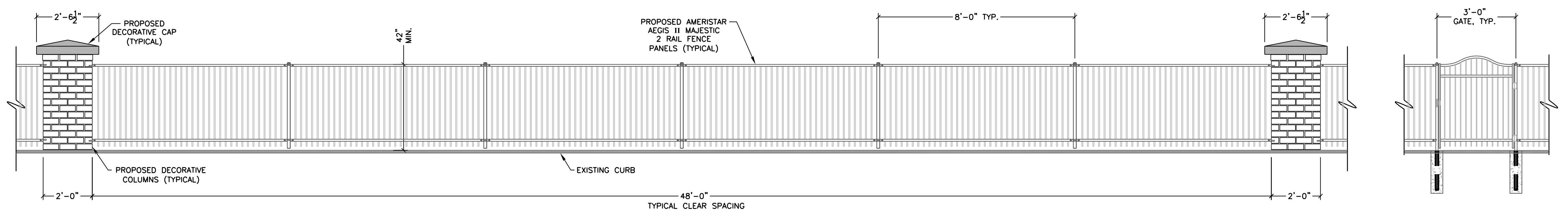
TYPICAL FENCE ELEVATION SCALE: 3/8"=1'-0"
