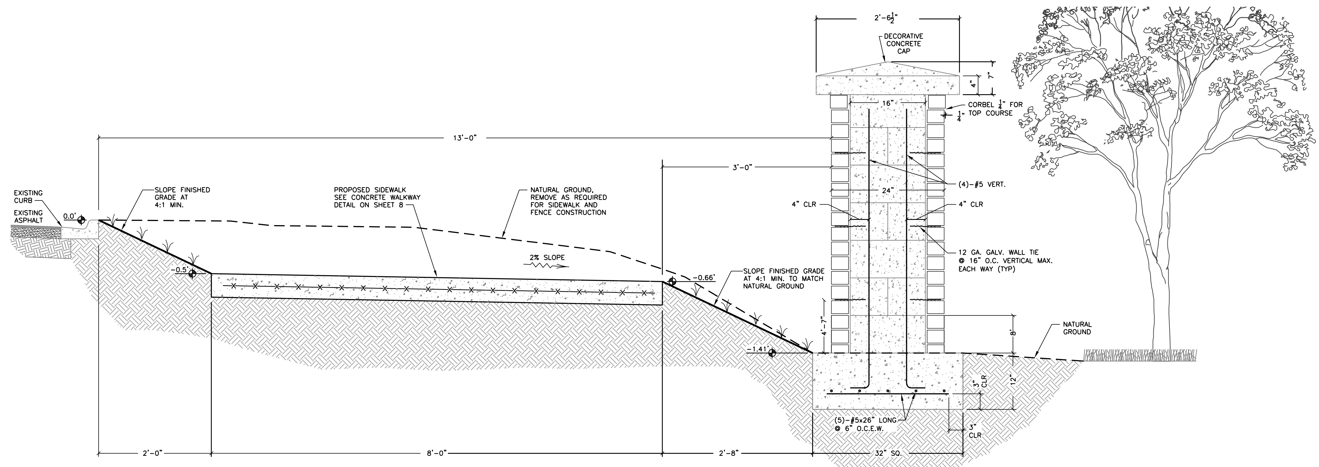
TYPICAL COLUMN SECTION STATIONS 11+00 THRU 27+00 SCALE: 1"=1'-0"
