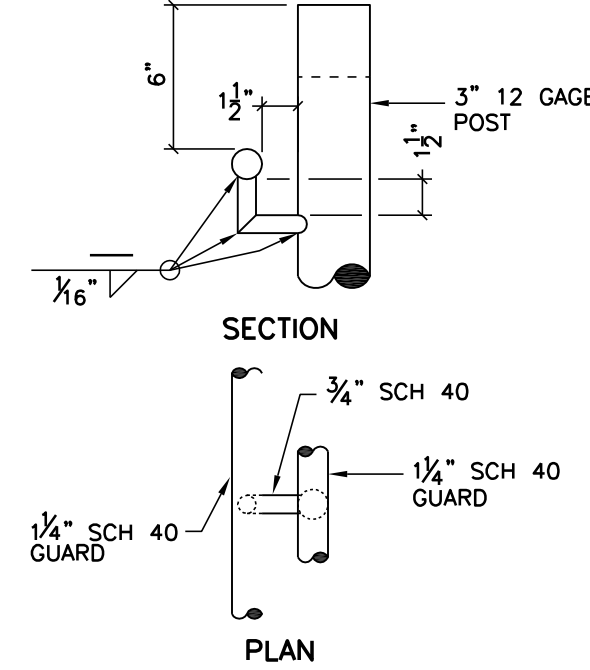
TYPICAL HANDRAIL DETAIL SCALE: 1 1/2"=1'-0"
