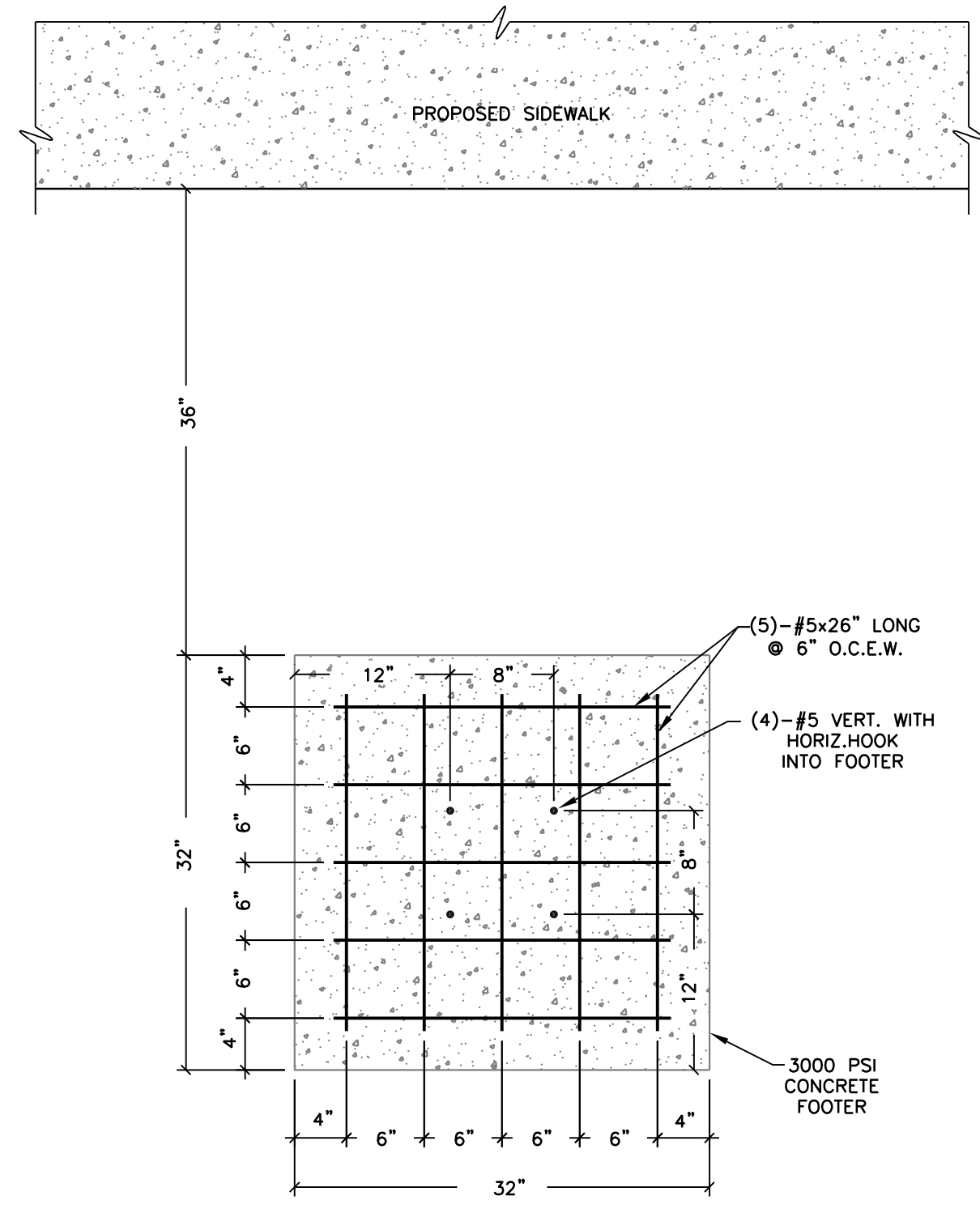
COLUMN FOUNDATION PLAN VIEW SCALE: 1"=1'-0"
