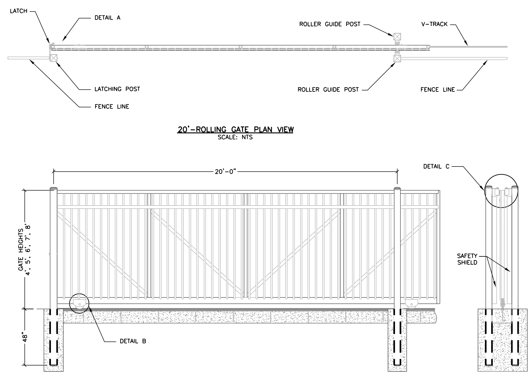
20'-ROLLING GATE ELEVATION SCALE: NTS
