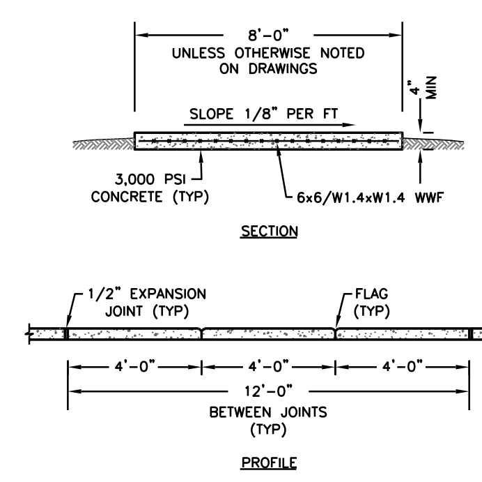
CONCRETE WALKWAY DETAIL NOT TO SCALE
