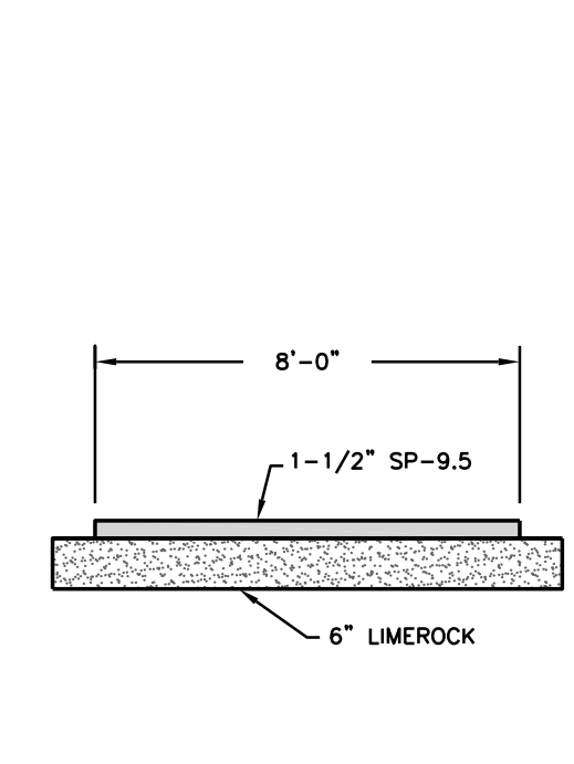
ASPHALT WALKWAY DETAIL NOT TO SCALE
