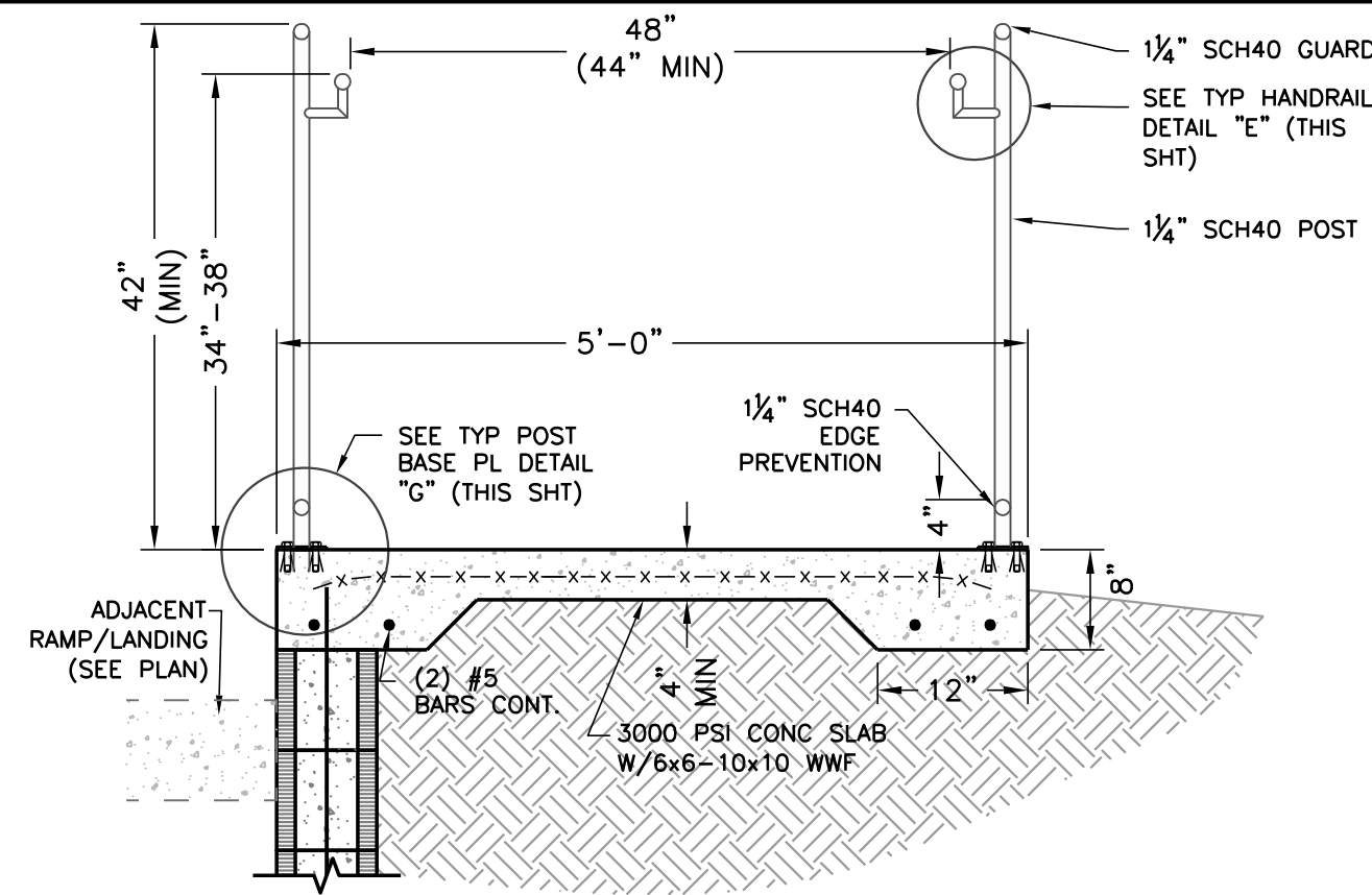
TYPICAL STAIR SECTION SCALE: 3/4"=1'-0"
