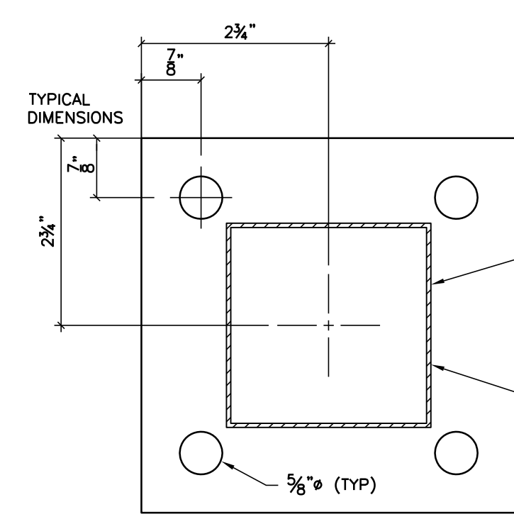
TYPICAL POST BASE PL DETAIL SCALE: 6"=1'-0"
