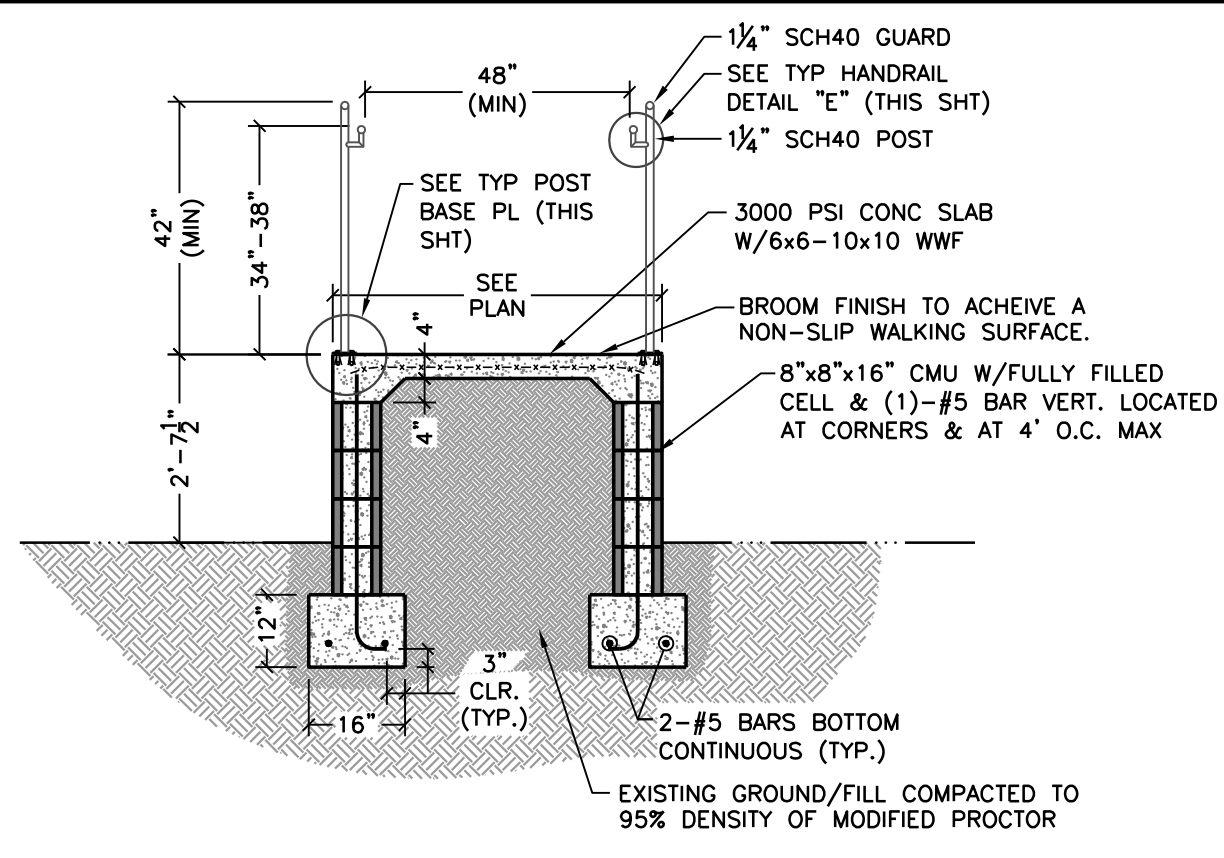
TYPICAL TOP LANDING SECTION SCALE: 3/8"=1'-0"
