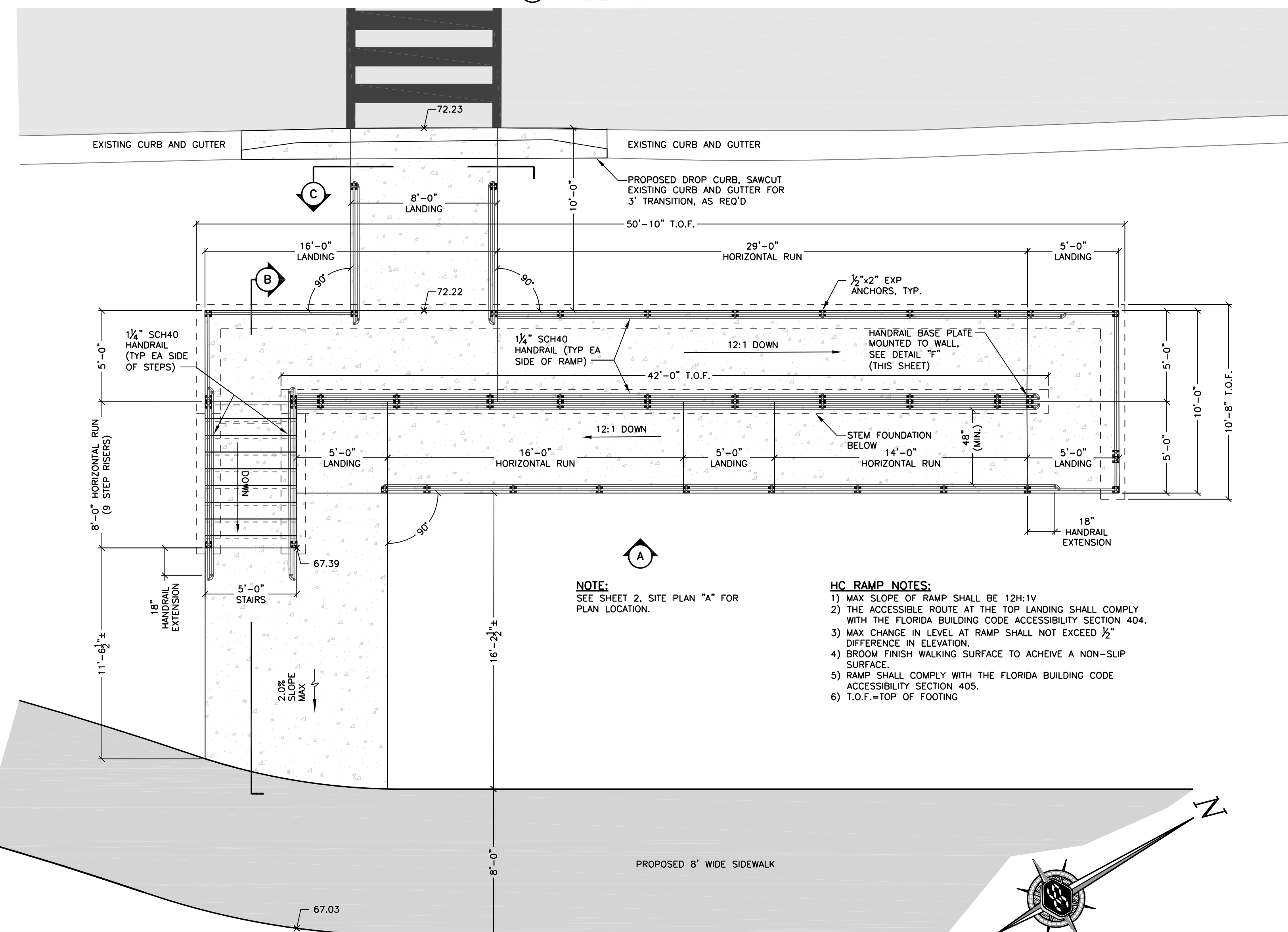
RAMP PLAN SCALE: 1"=5'-0"
