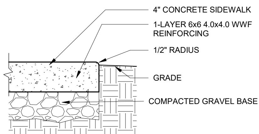
3 SIDEWALK EDGE 1 1/2" = 1'-0"
