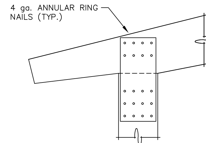
COLUMN TO BEAM CONNECTION
