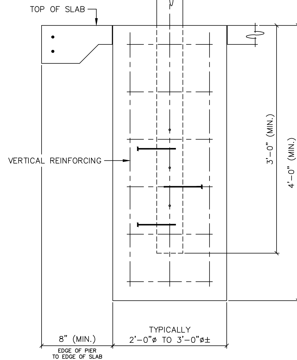
COLUMN PIER DETAIL
