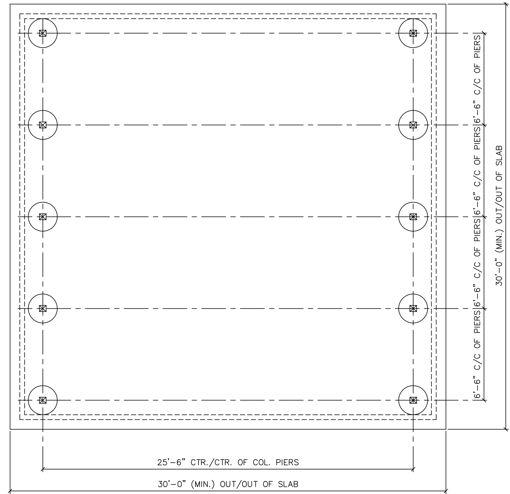
FOUNDATION PLAN
