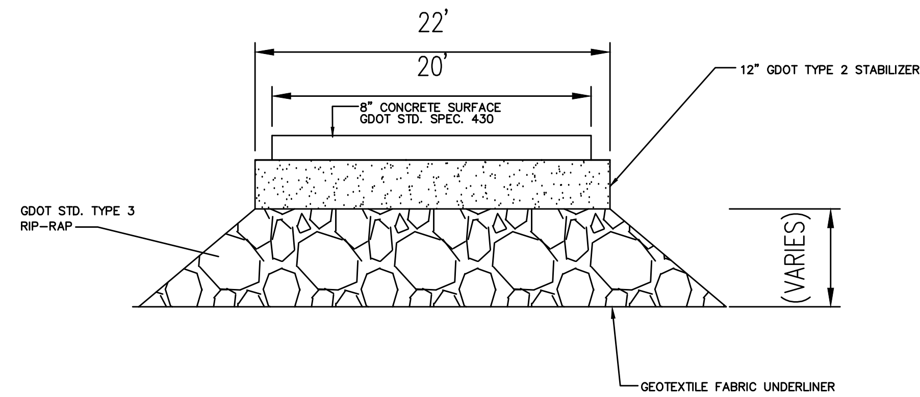
BOAT RAMP CROSS SECTION
