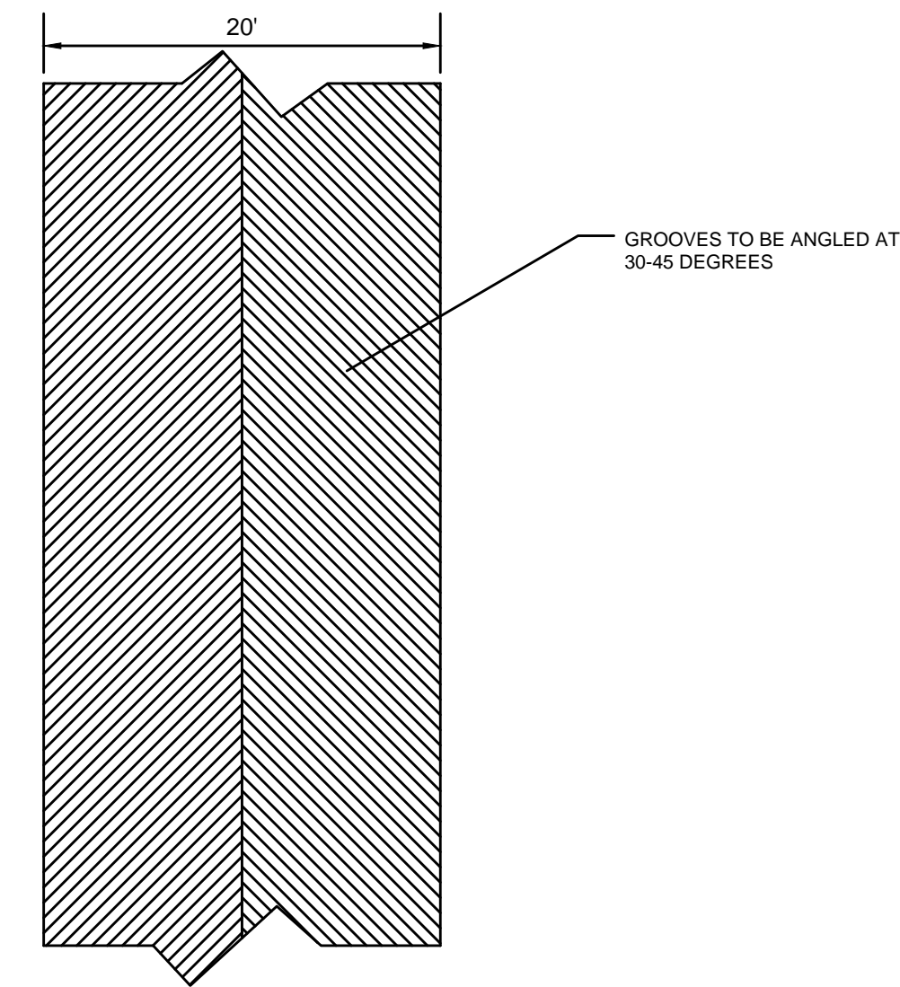
PLAN VIEW OF PUSH SLAB (WITH CHEVRON-STYLE GROOVING)
