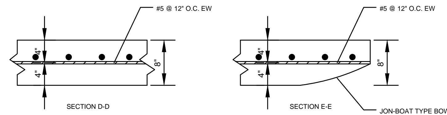
SUBMERGED BOAT RAMP SECTION (PUSH SLAB)
