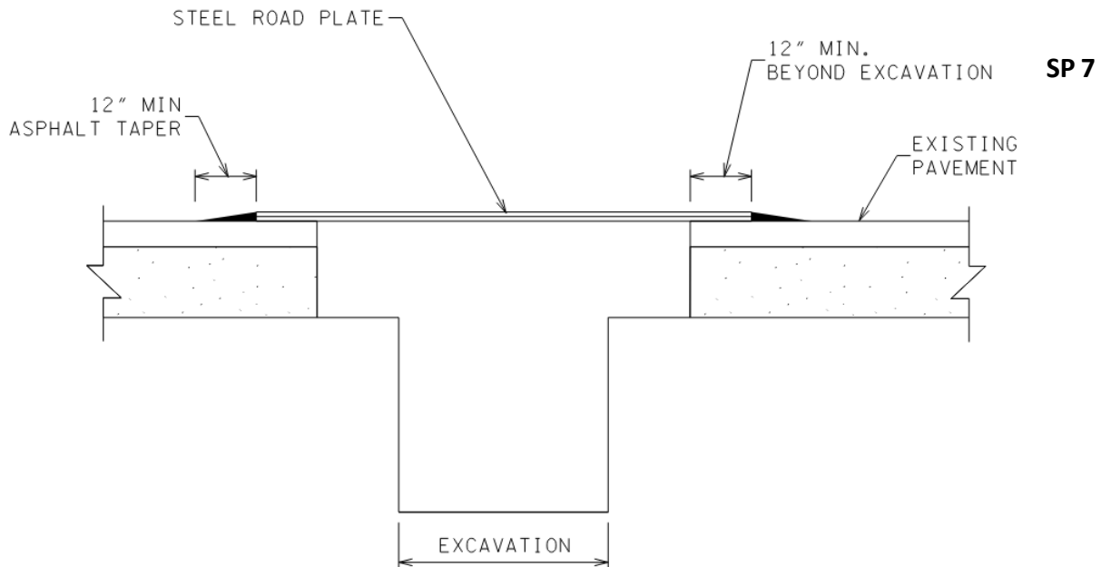
STEEL ROAD PLATE DETAIL
