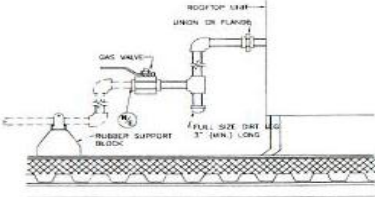
ROOFTOP GAS CONNECTION DETAIL 3 SCHEMATIC
