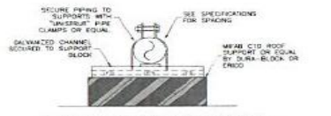
ROOFTOP GAS PIPING SUPPORT 2 SCHEMATIC
