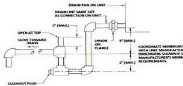
CONDENSATE DRAIN TRAP DETAIL 1 NOT TO SCALE
