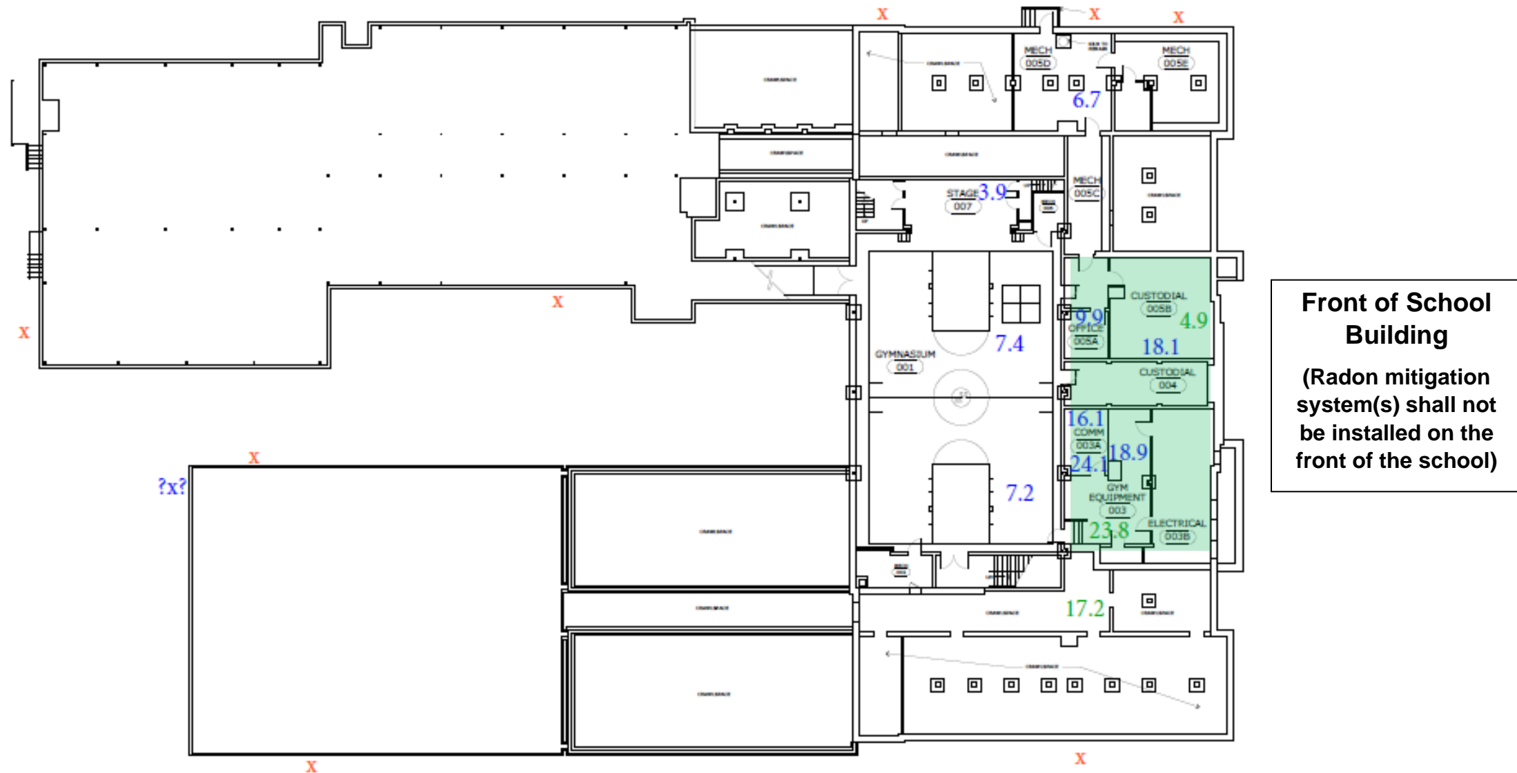
Figure 1: Targeted areas of Russell Cave Elementary School for ASD Radon Mitigation (Green). X - Current Radon Mitigation Systems 11 – 2021-2022 Radon Measurements Slab A above corresponds to the suction point in Appendix A: Radon Diagnostic Report.
