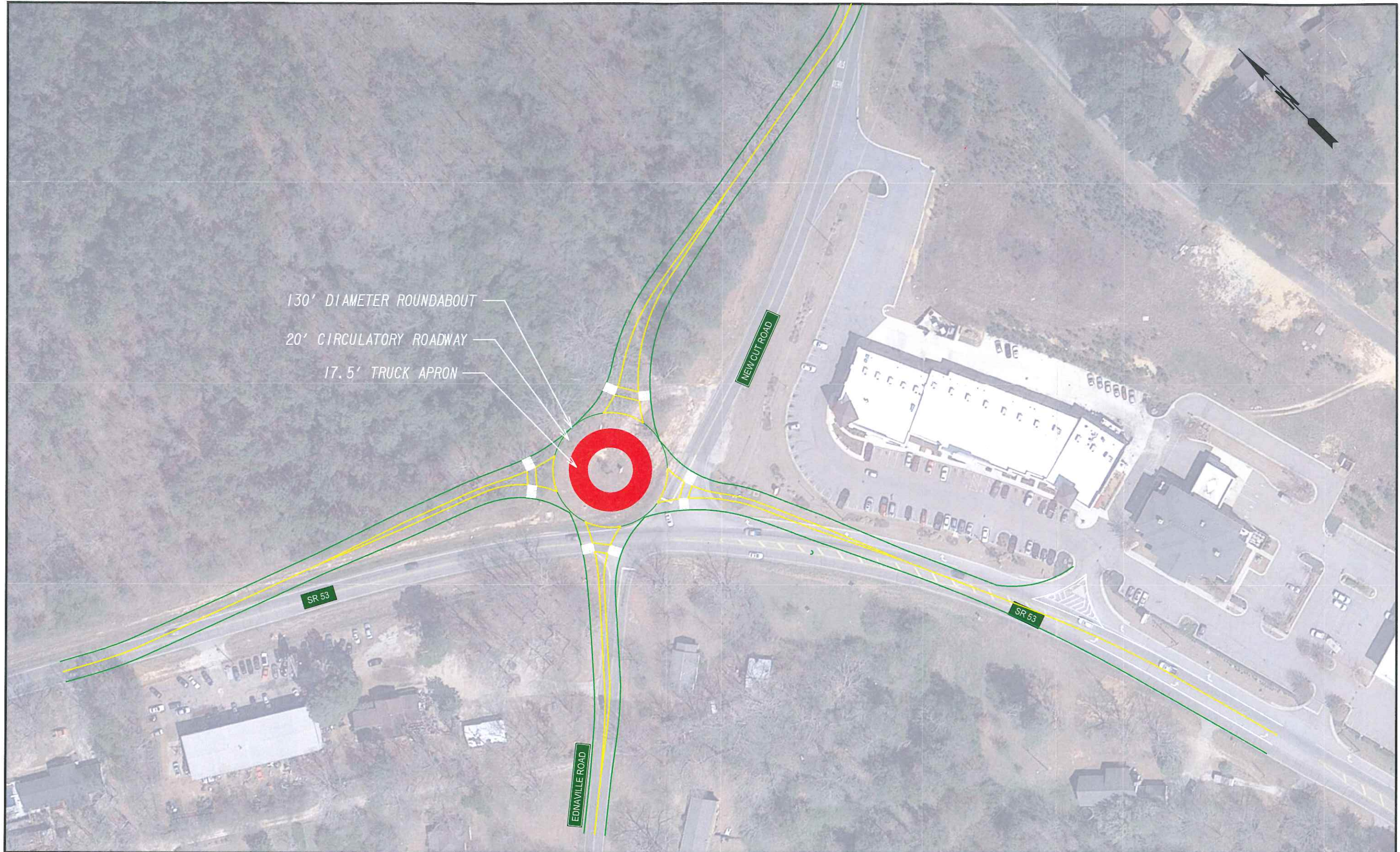
SR 53 @ NEW CUT RD ROUNDABOUT DESIGN
