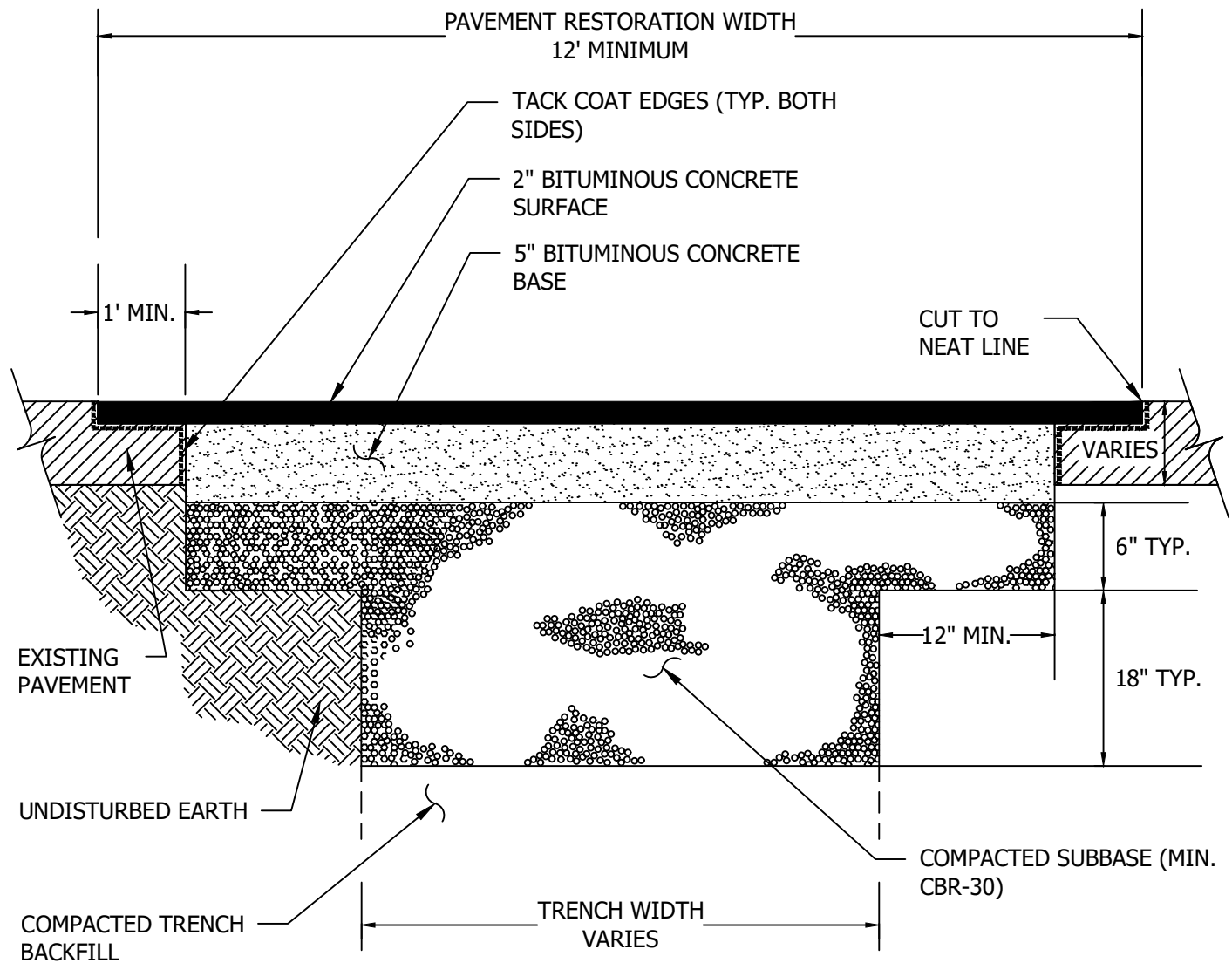
TYPICAL SECTION
