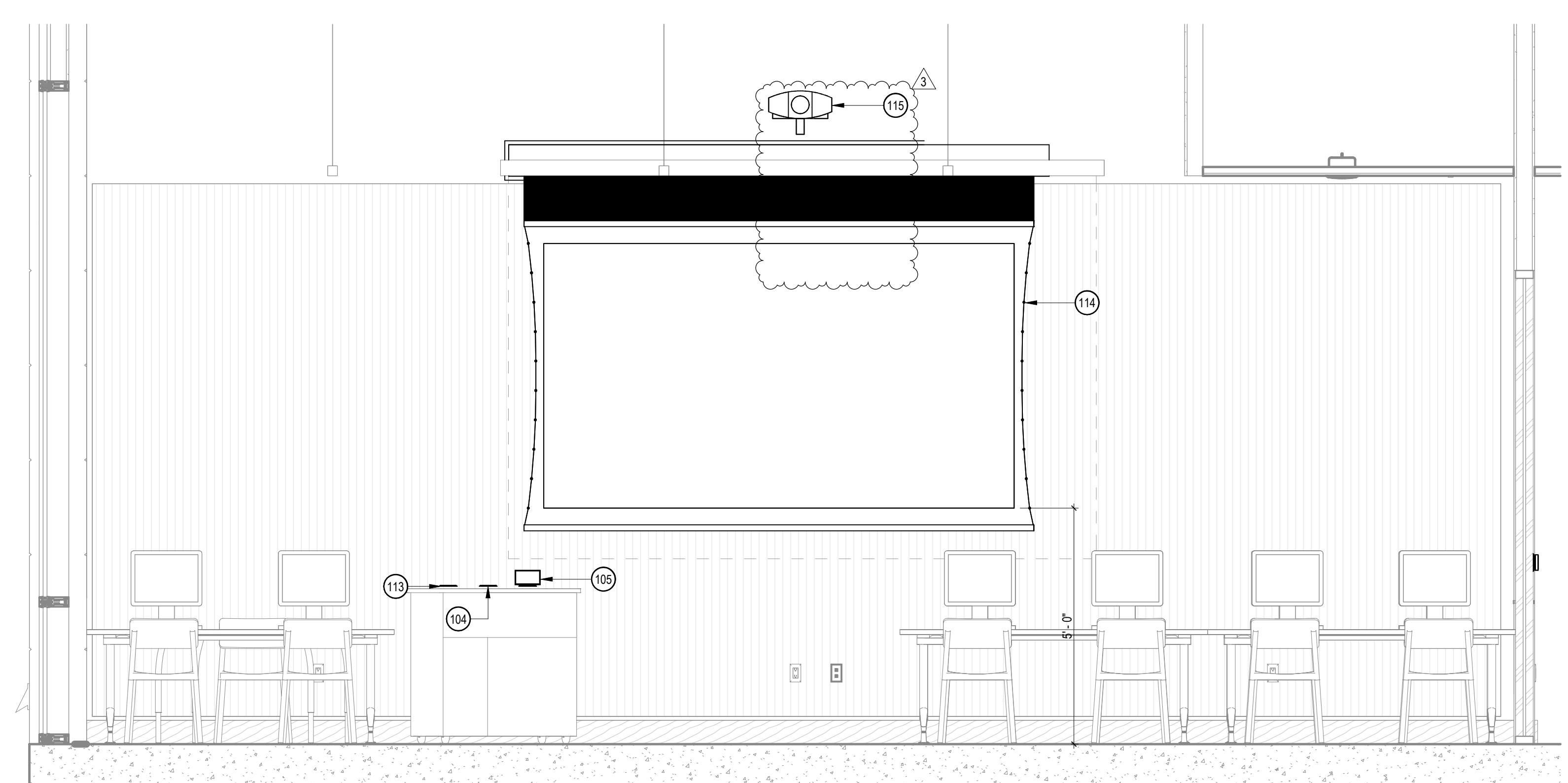
5 EQUIPMENT ELEVATION
