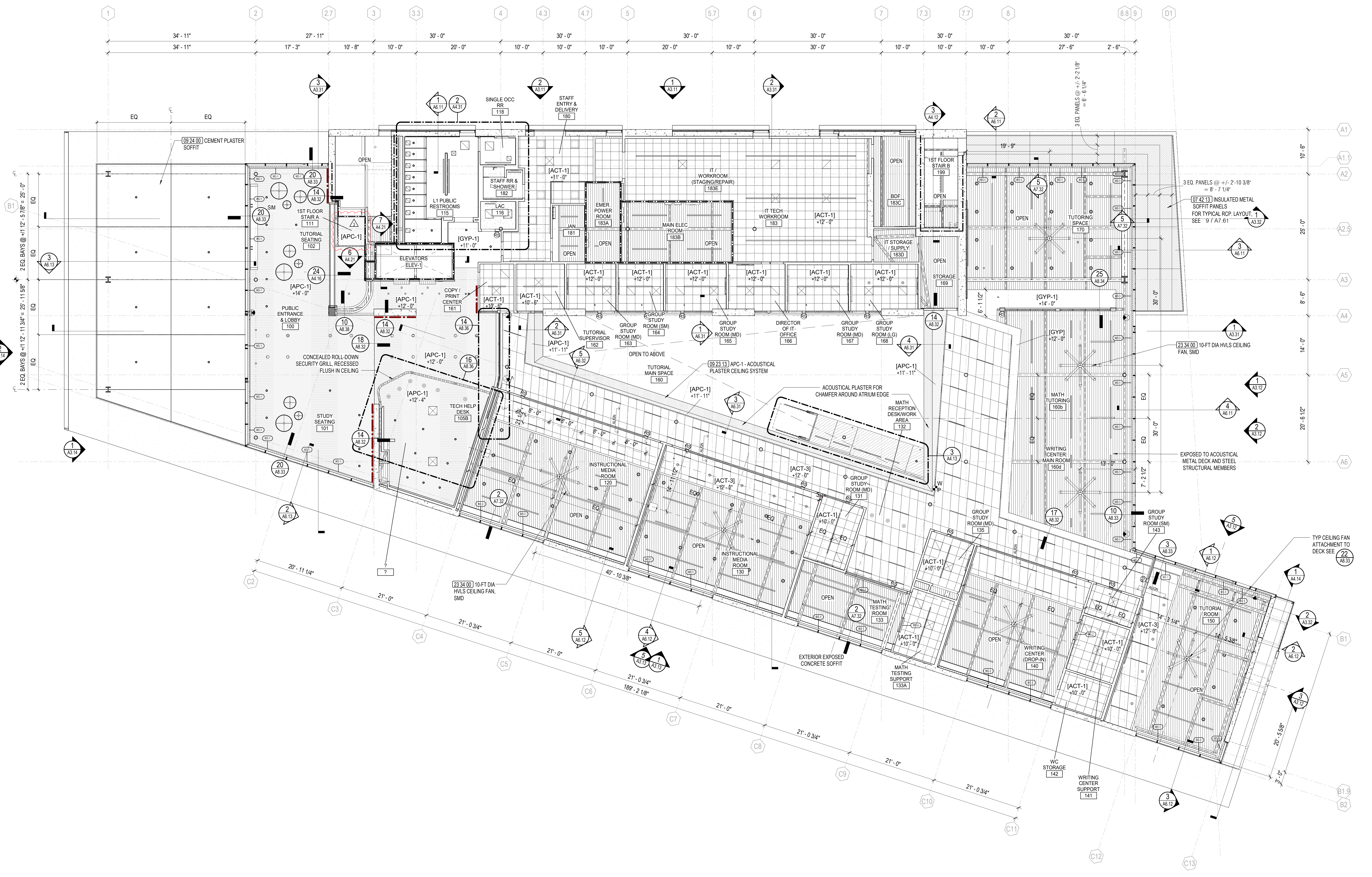
01 - CEILING PLAN 1/8" = 1'-0"
