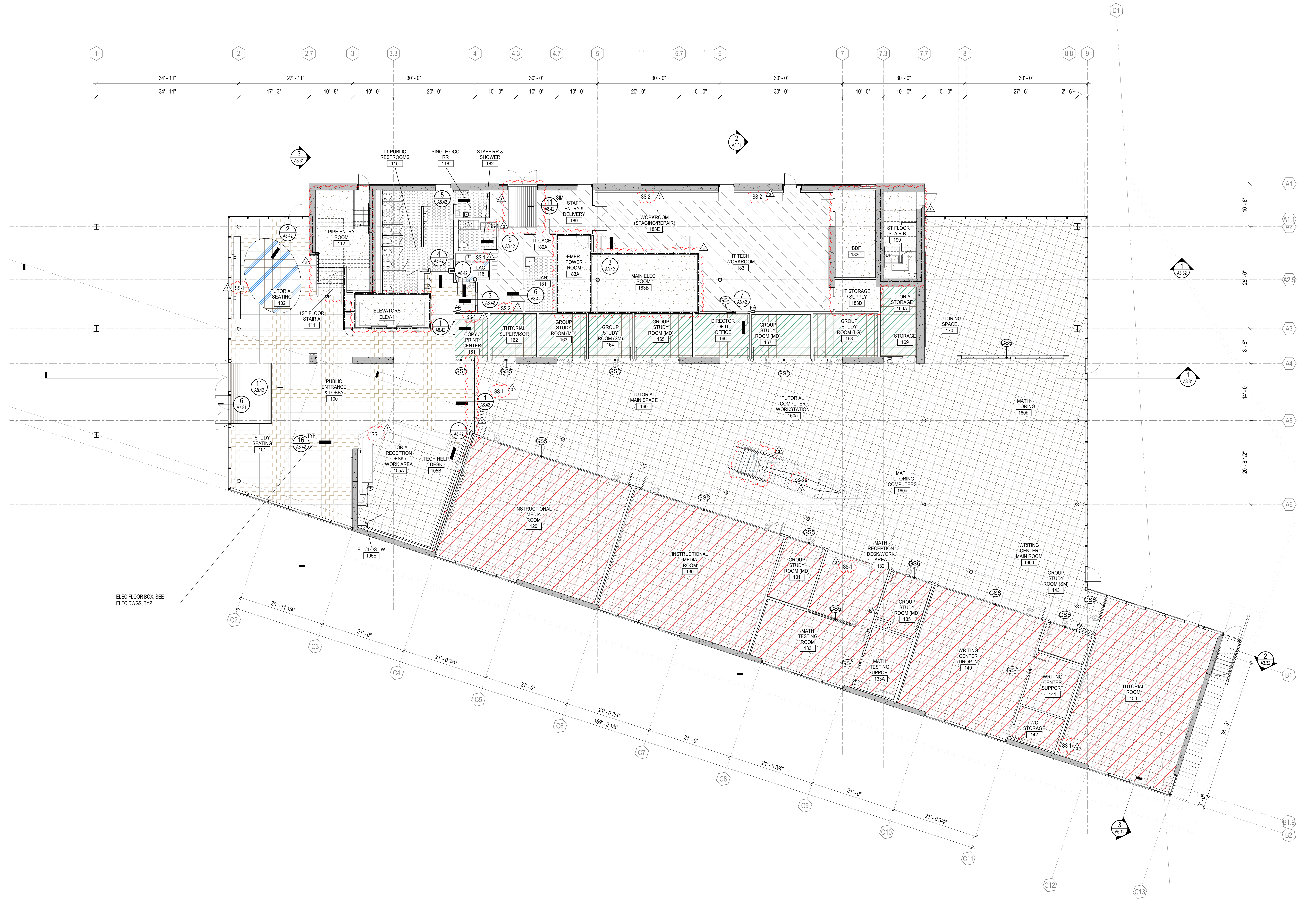
01 - FINISH PLAN 1/8" = 1'-0"
