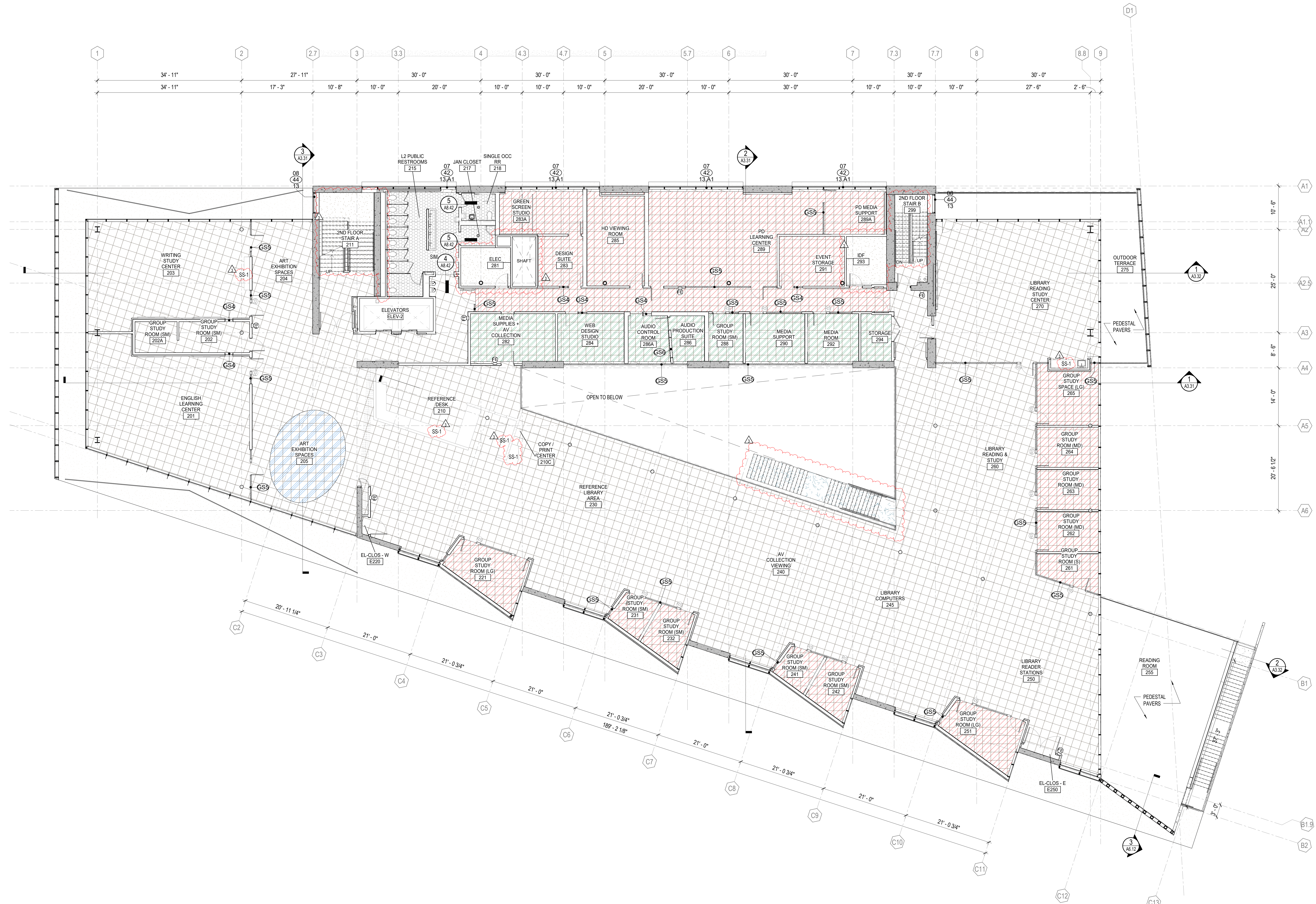
02 - FINISH PLAN 1/8" = 1'-0"
