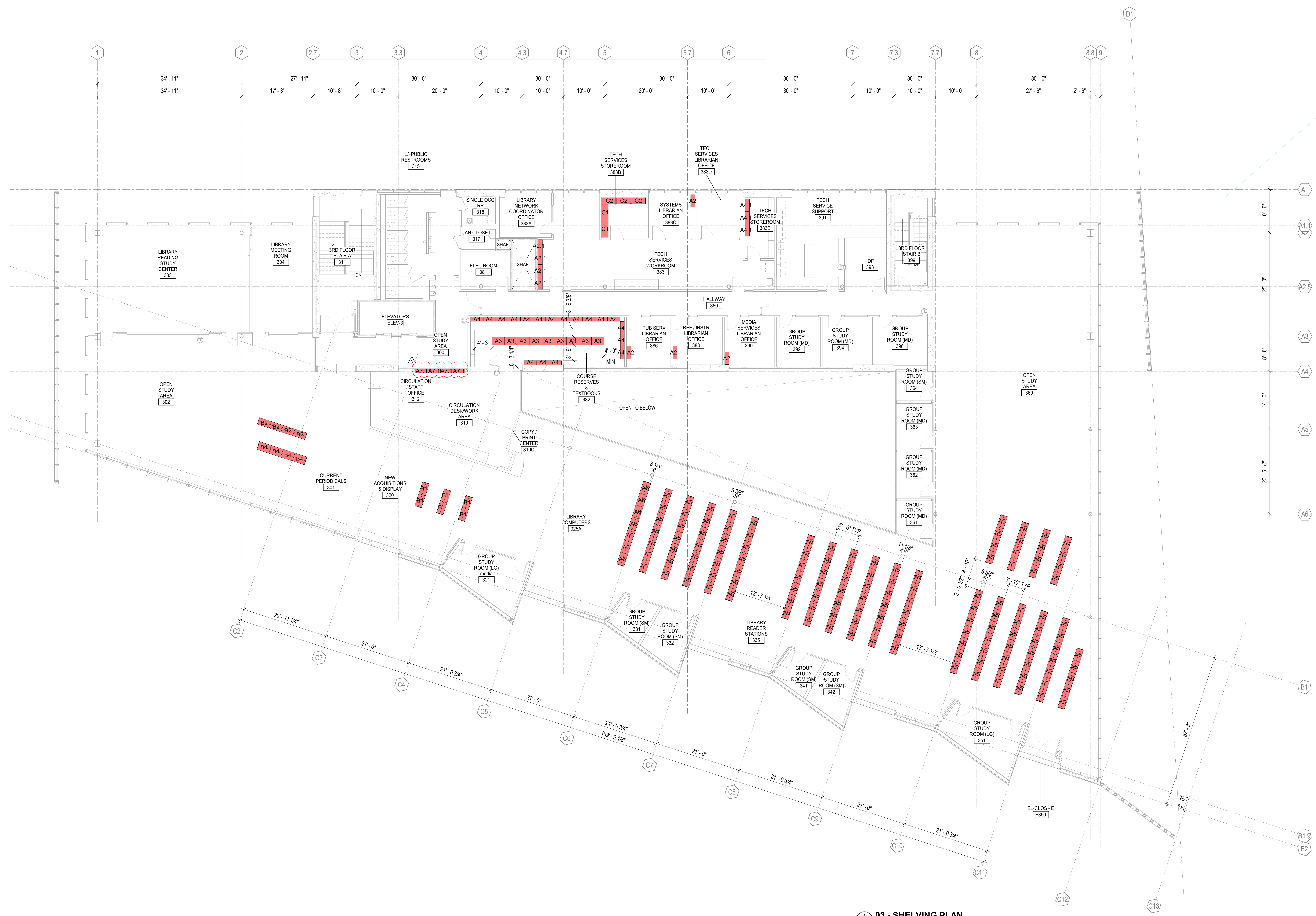
03 - SHELVING PLAN 1/8" = 1'-0"
