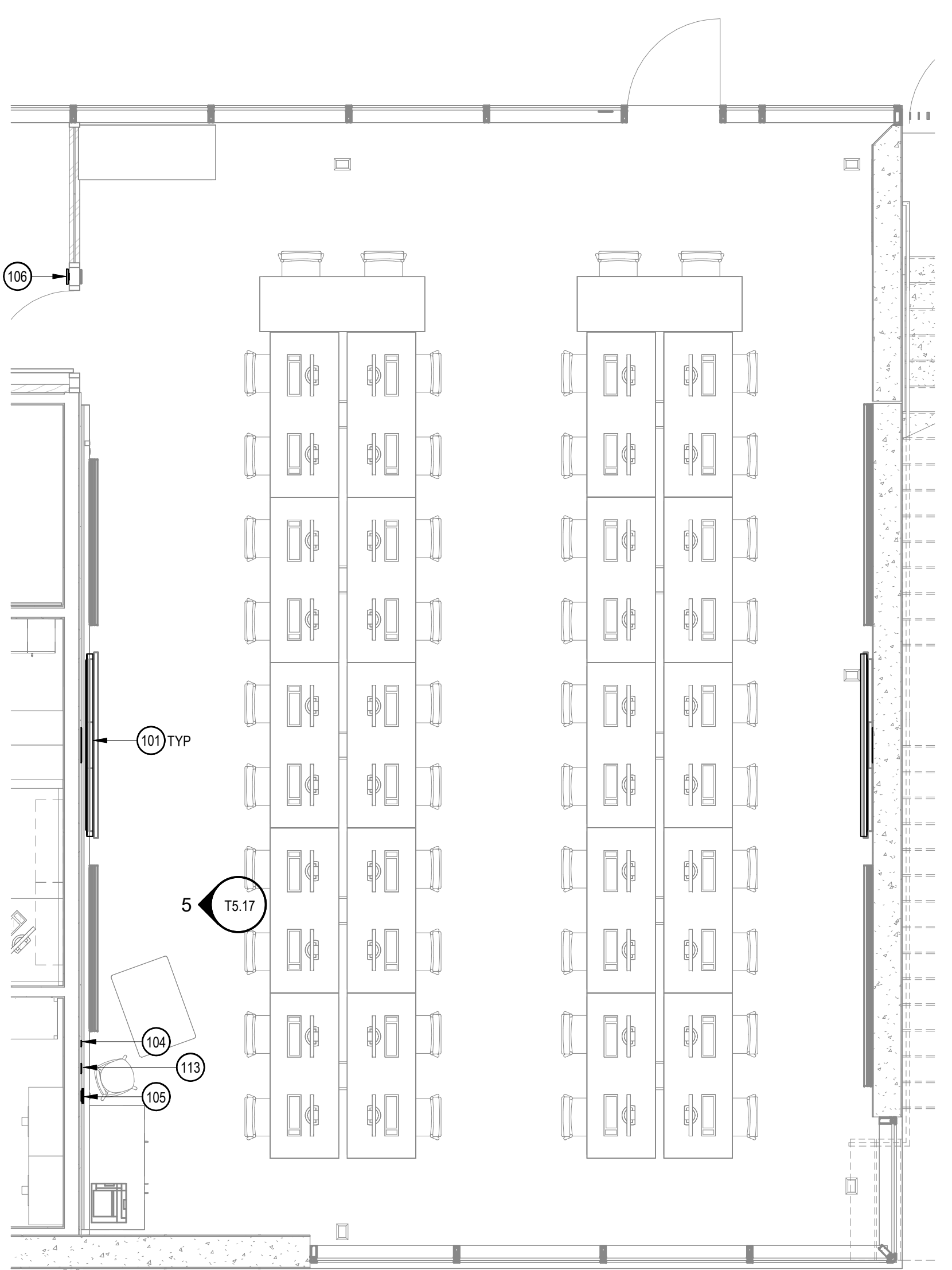
2 EQUIPMENT PLAN SCALE: 1/4" = 1'-0"
