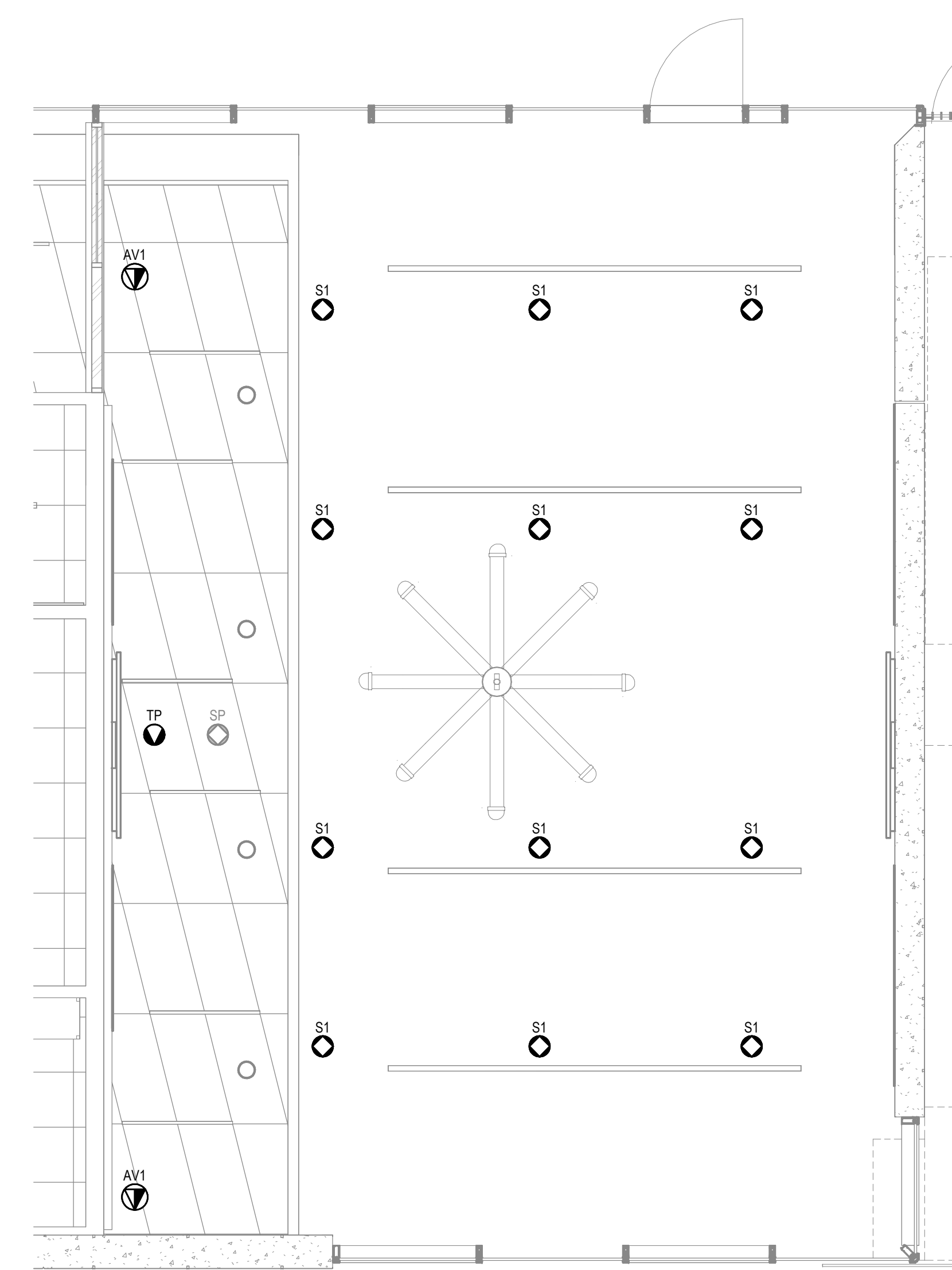
3 REFLECTED CEILING PLAN SCALE: 1/4" = 1'-0"
