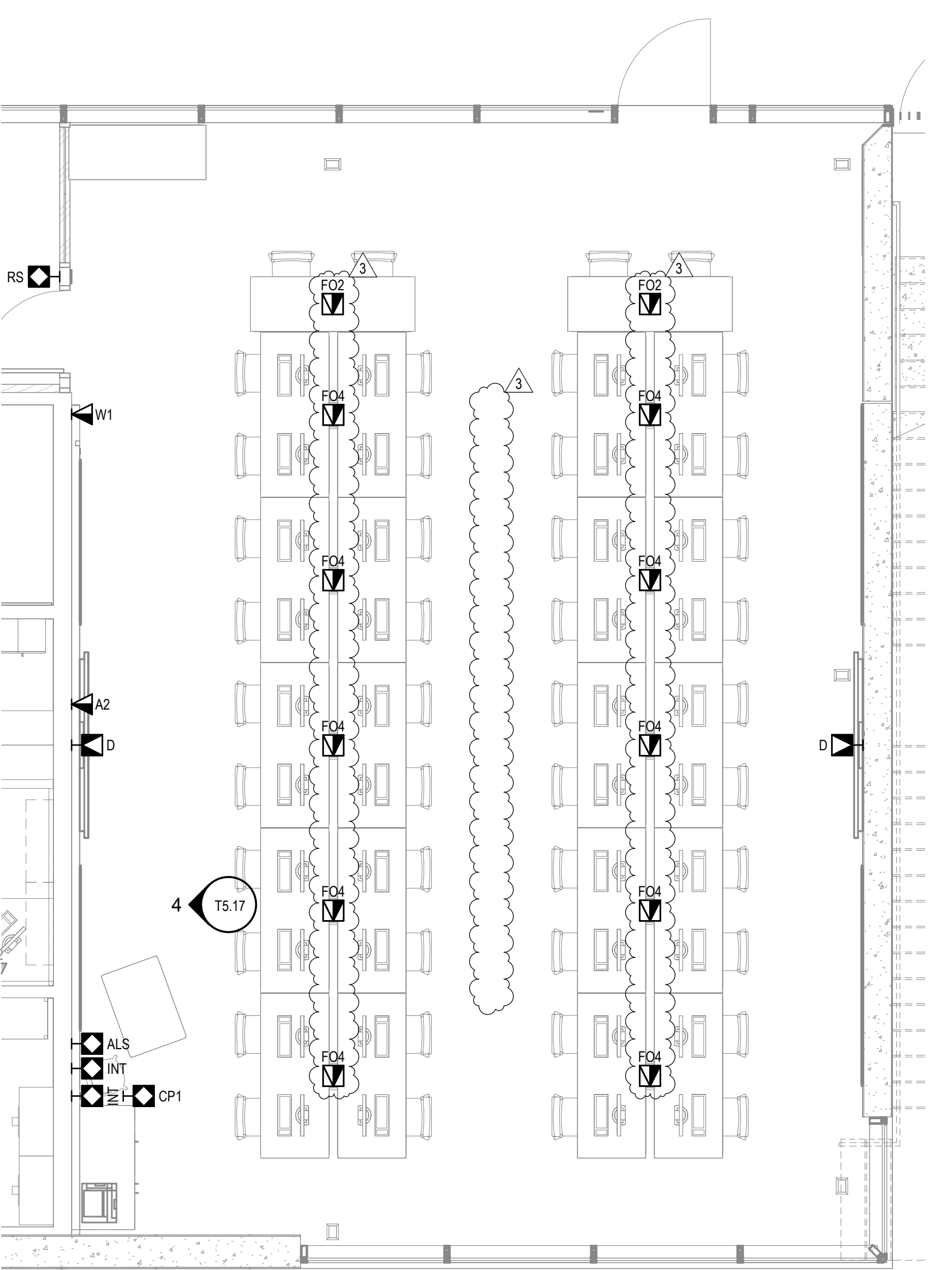
1 INFRASTRUCTURE PLAN SCALE: 1/4" = 1'-0"
