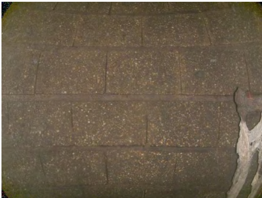
1838_4d464b94-a957-4557-a7ae-8bb14bf4d783_5c5b9007-ca65-4280-add5-f176f9132037_P11.jpg, 00:00:28, 6.15 Missing Mortar Large from 12 o'clock to 12 o'clock
