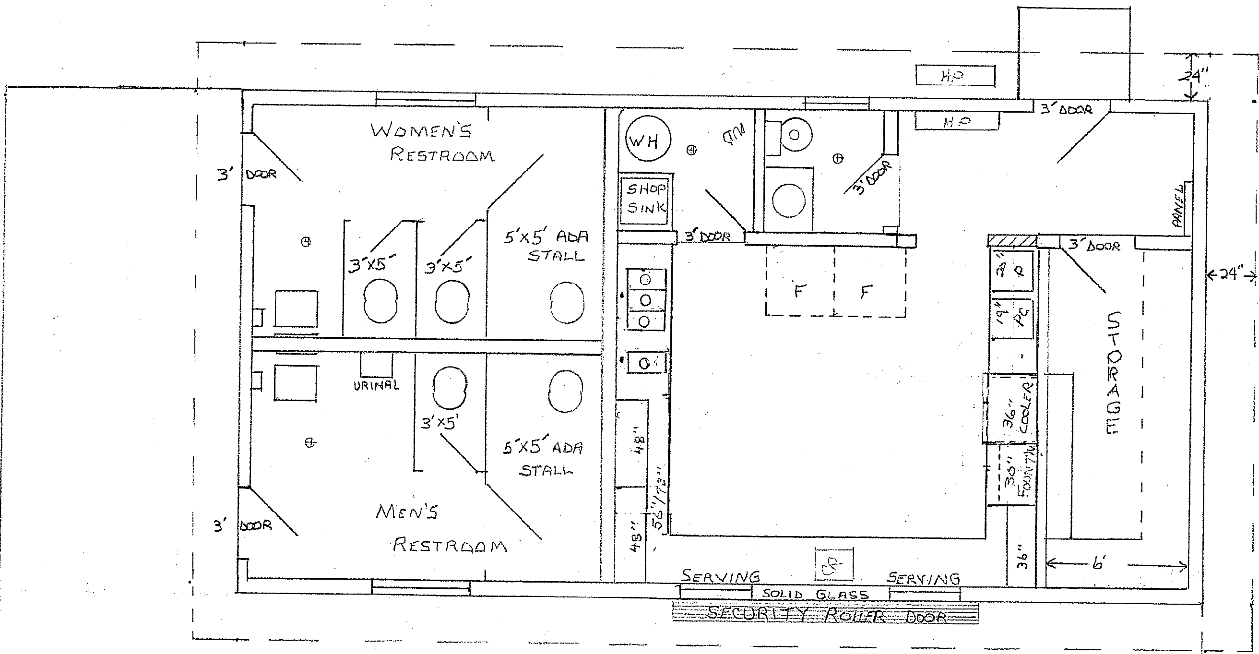
FLOOR PLAN
