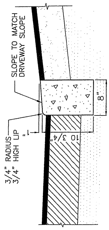
6" DROP CURB AT ASPHALT DRIVEWAY
