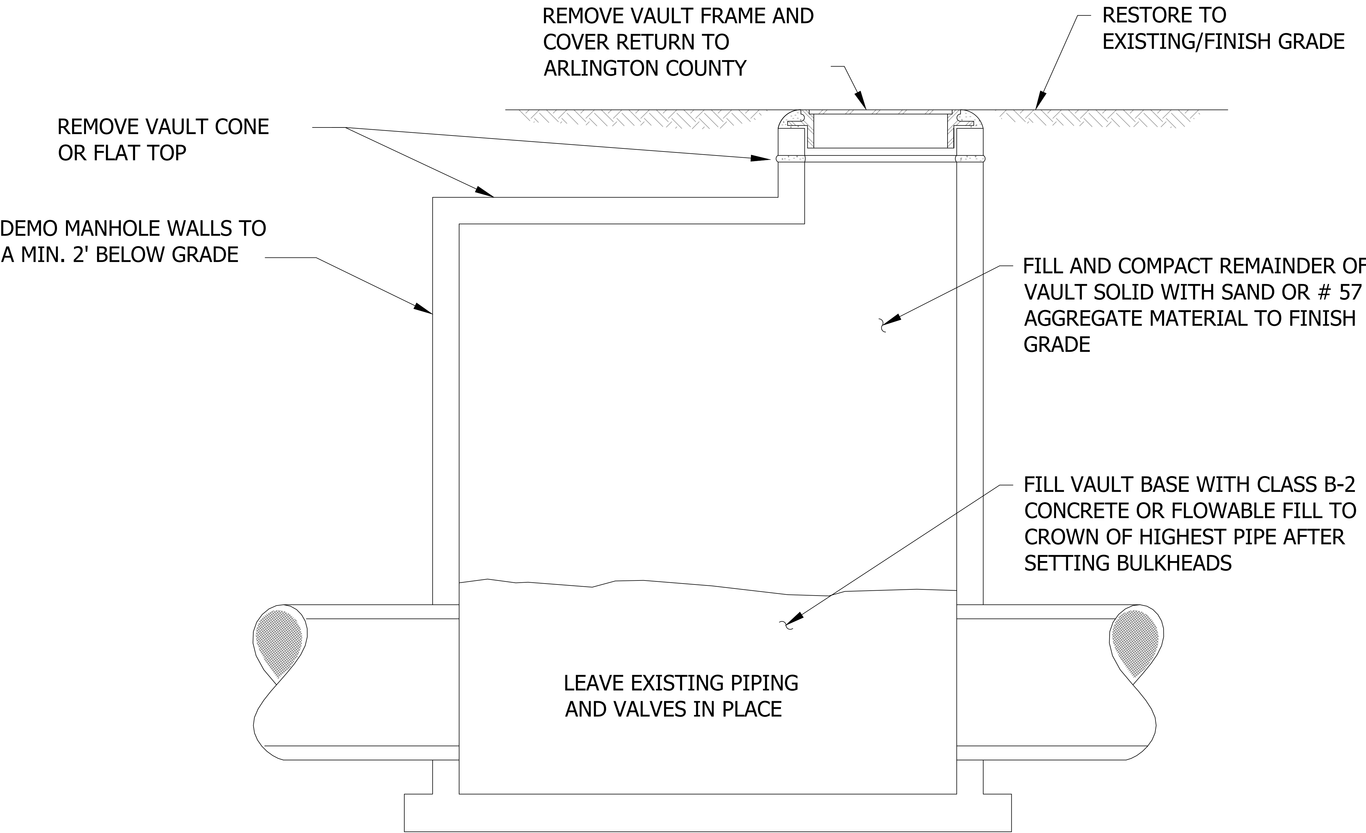
6 EXISTING VAULT ABANDONMENT DETAIL N.T.S.
