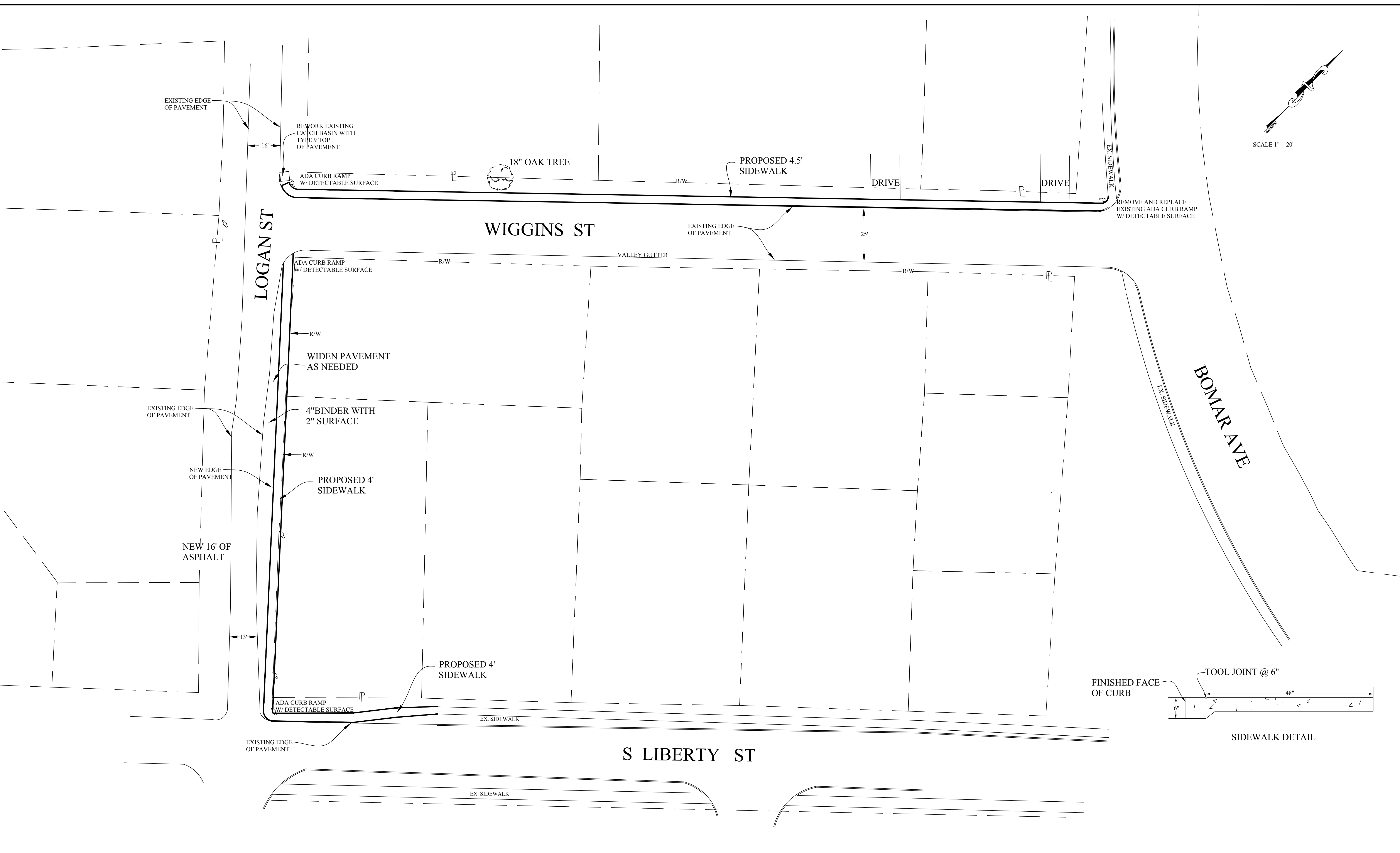
S. LIBERTY STEET, LOGAN STREET WIGGINS STEET SIDEWALK PROJECT
