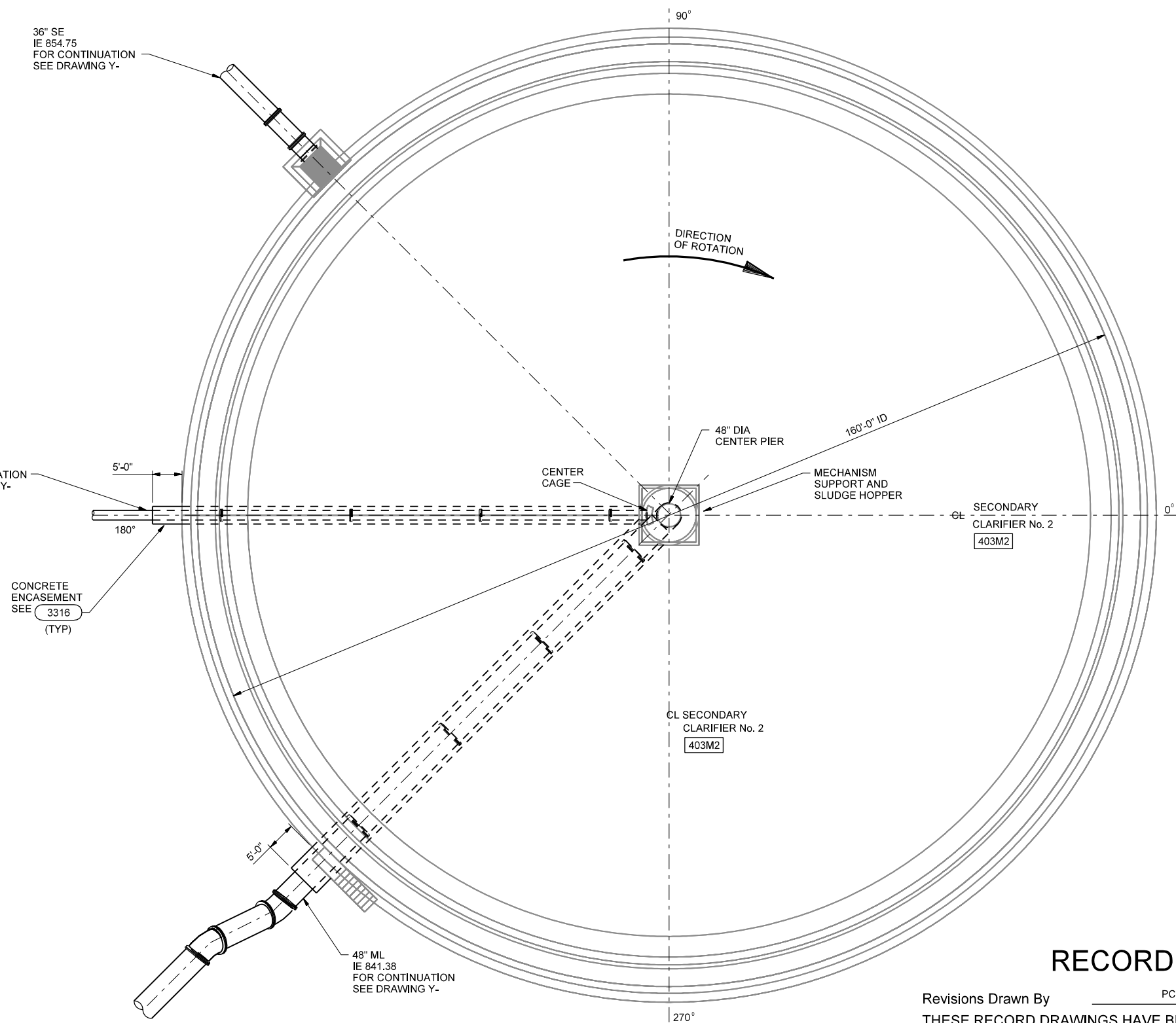
PLAN 3/32" = 1'-0"
