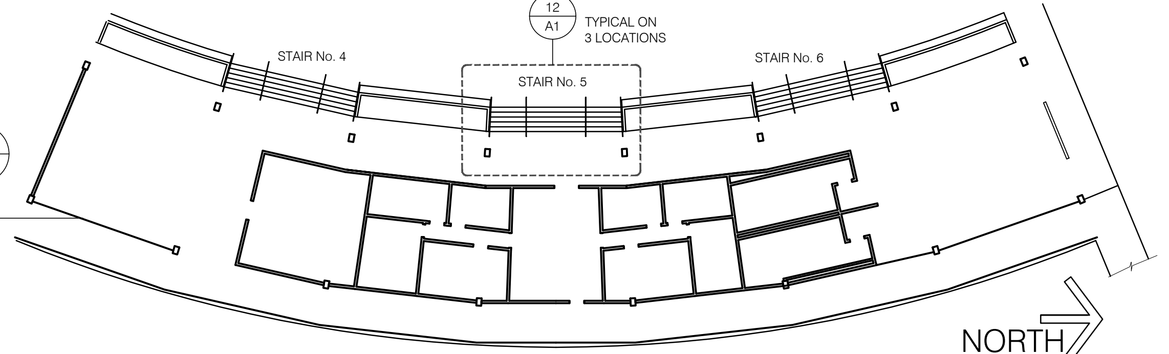
3 FLOOR PLAN BUILDING 100 WEST WING SCALE: 1" = 20"
