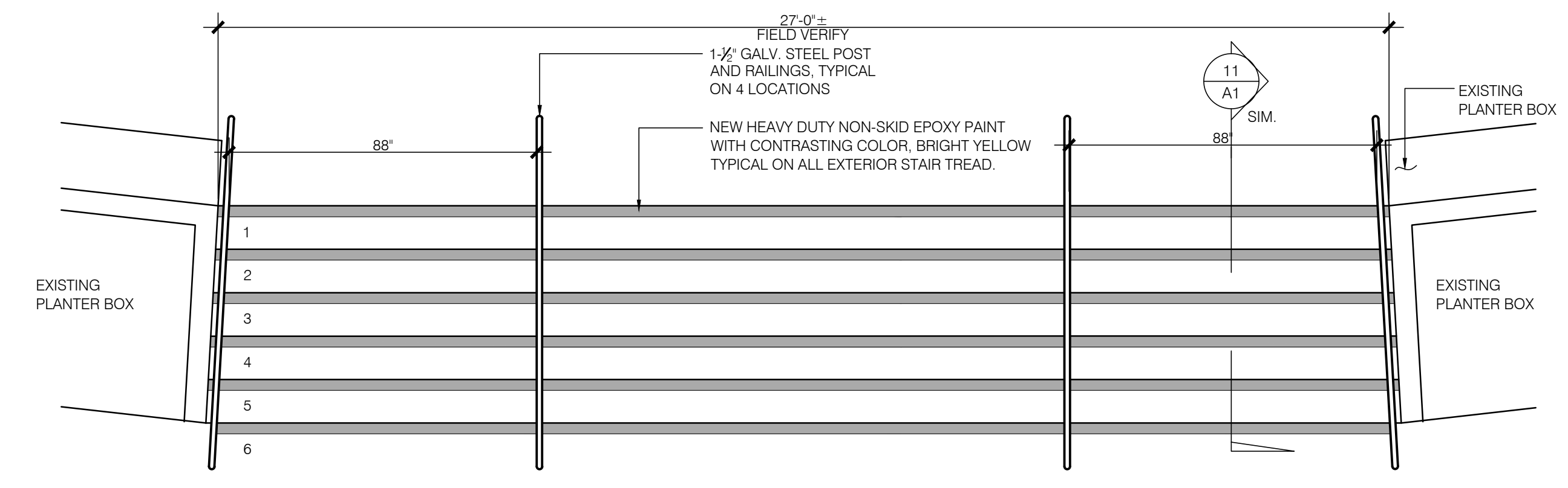
12 TYPICAL STAIR PLAN BLDG. 100 WEST WING SCALE: 3/8" = 1'-0"
