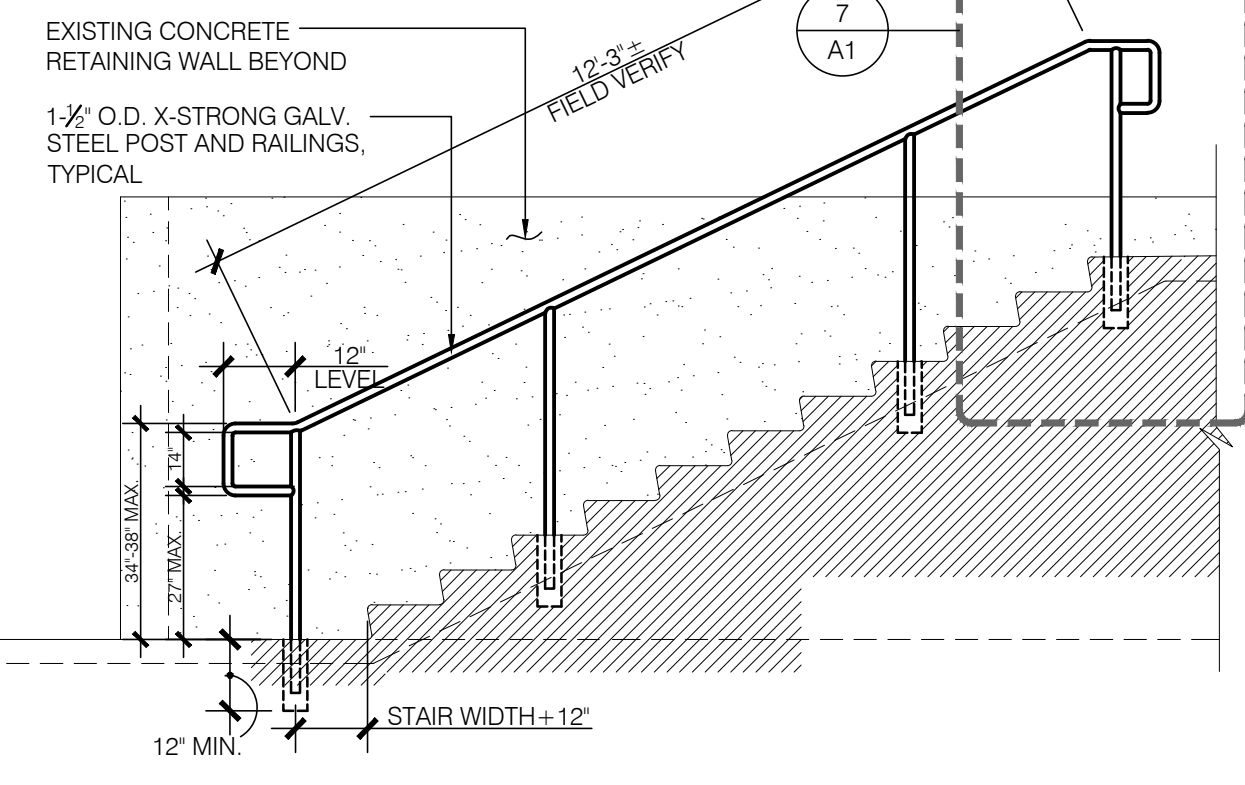
11 TYPICAL STAIR SECTION SCALE: 3/8" = 1'-0"
