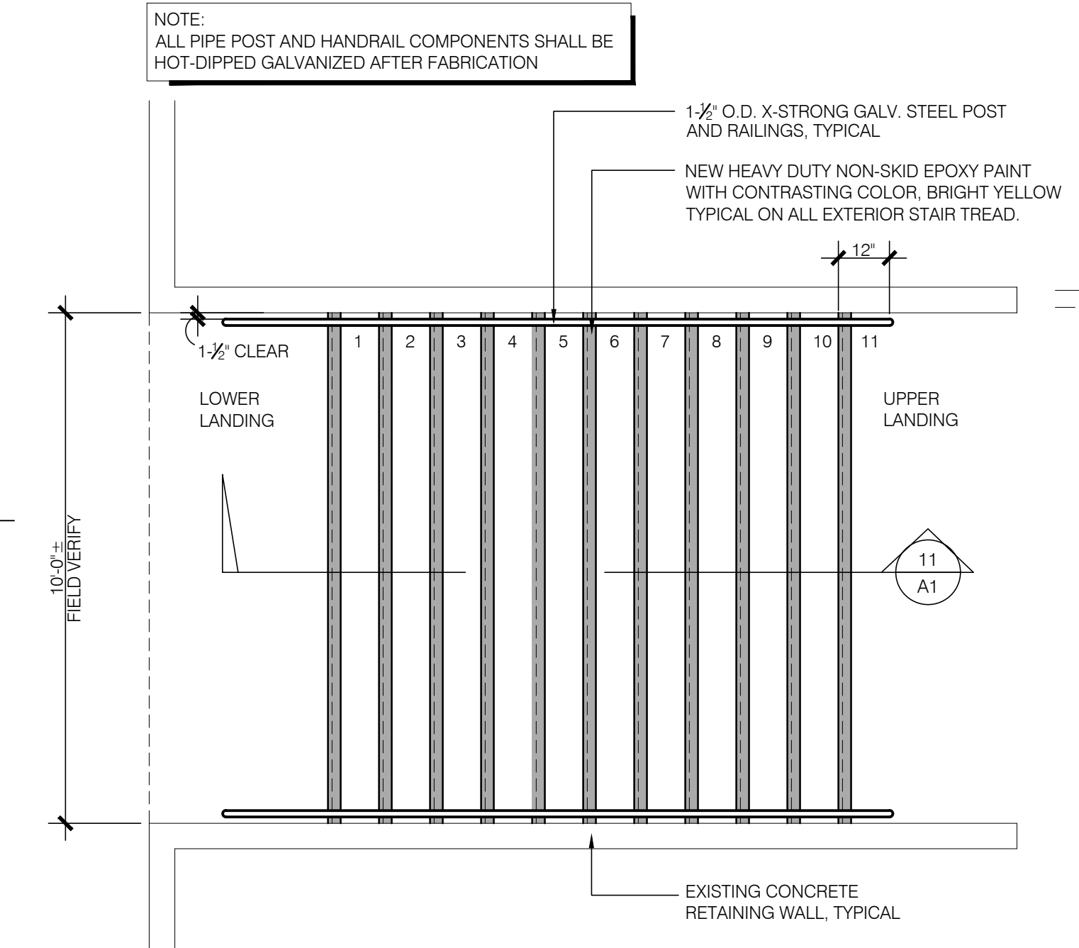
16 TYPICAL STAIR PLAN BLDG. AD-1 SCALE: 3/8" = 1'-0"
