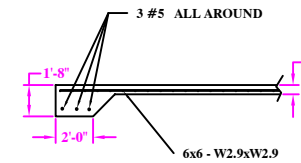
SLAB DETAIL
