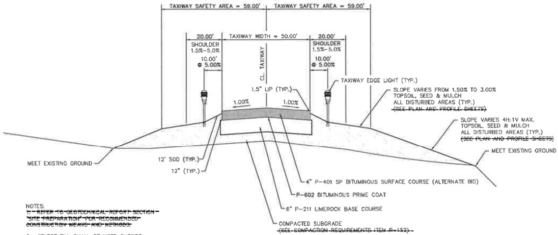
TYPICAL TAXIWAY SECTION NOT TO SCALE
