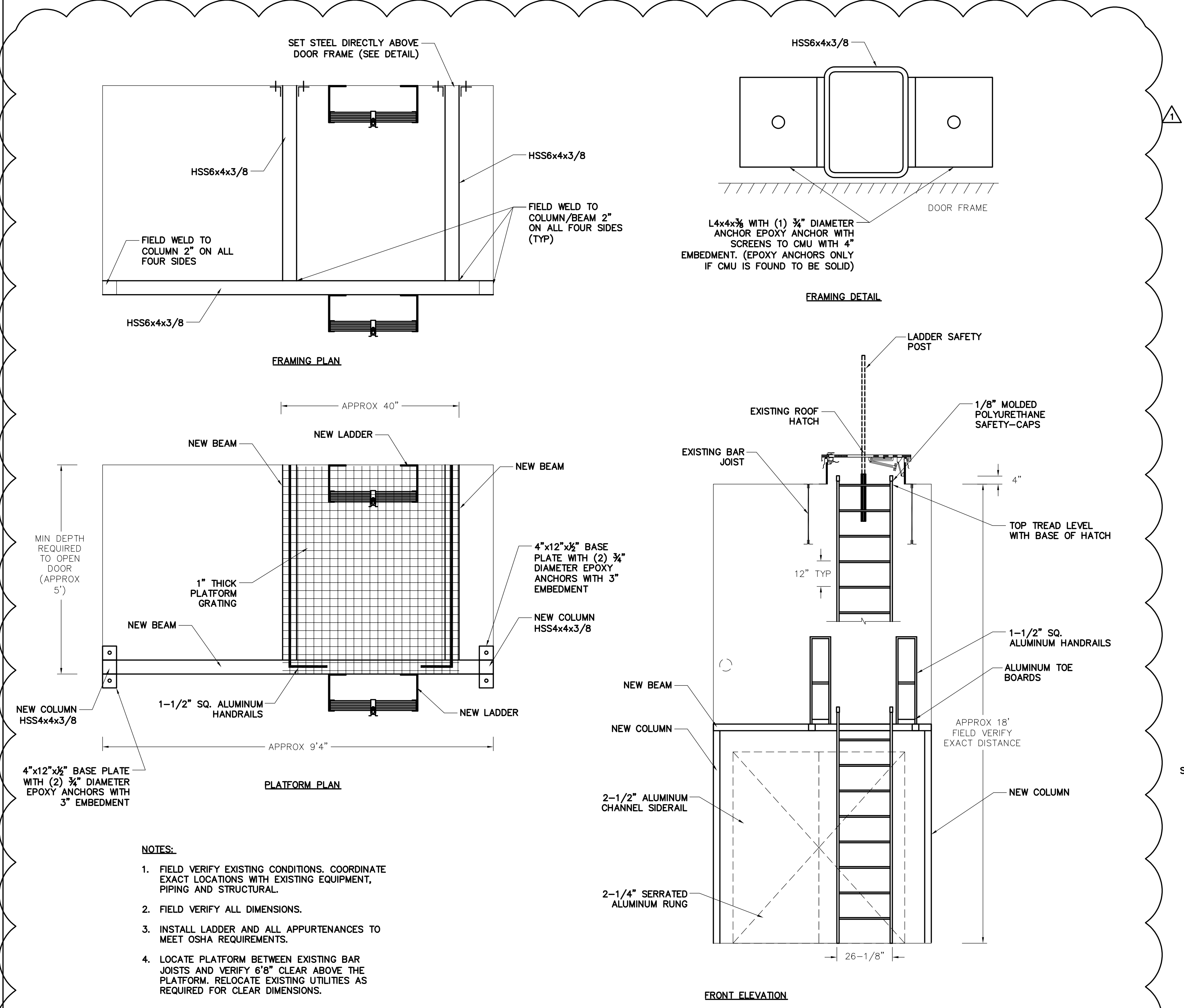
2 LADDER #1 DETAIL GC104 SCALE: NTS
