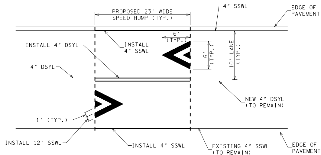
PROPOSED SPEED HUMP PAVEMENT MARKING DETAIL NOT TO SCALE
