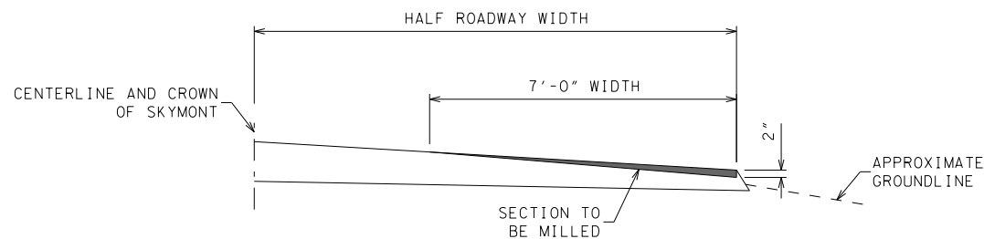
HALF SECTION FOR EDGE MILLING NOT TO SCALE
