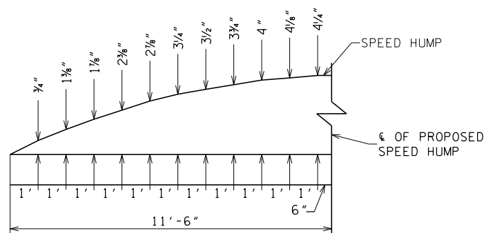
HALF SECTION NOT TO SCALE
