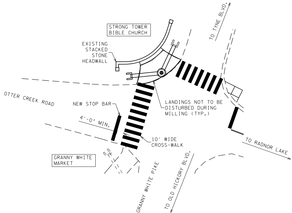
PLAN VIEW SHOWING CROSS-WALK AT GRANNY WHITE PIKE NOT TO SCALE
