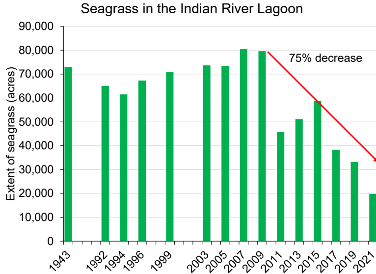
Figure 2. Seagrass extent mapped with aerial photography.
