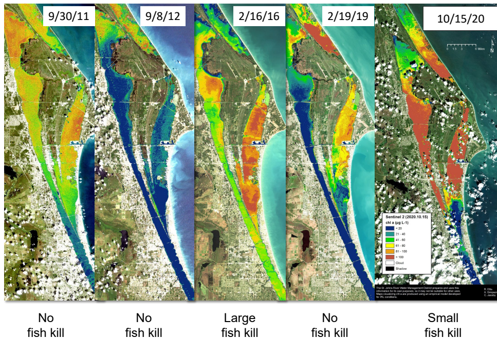
Figure 3. Concentrations of chlorophyll-a derived from satellite imagery, with annotations regarding fish kills.
