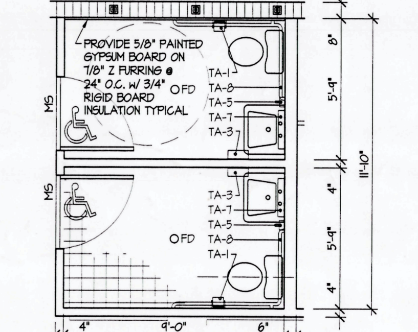
1 ENLARGED PLAN 1/4" = 1'-0"
