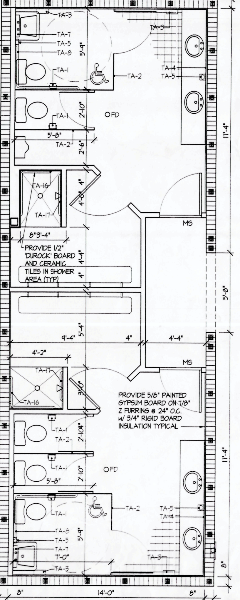
3 ENLARGED PLAN 1/4" = 1'-0"
