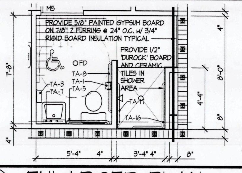
2 ENLARGED PLAN 1/4" = 1'-0"
