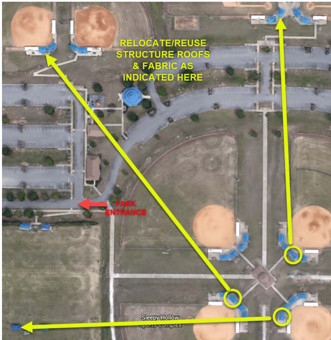
Figure b. Relocation of 3 Structure Roofs
