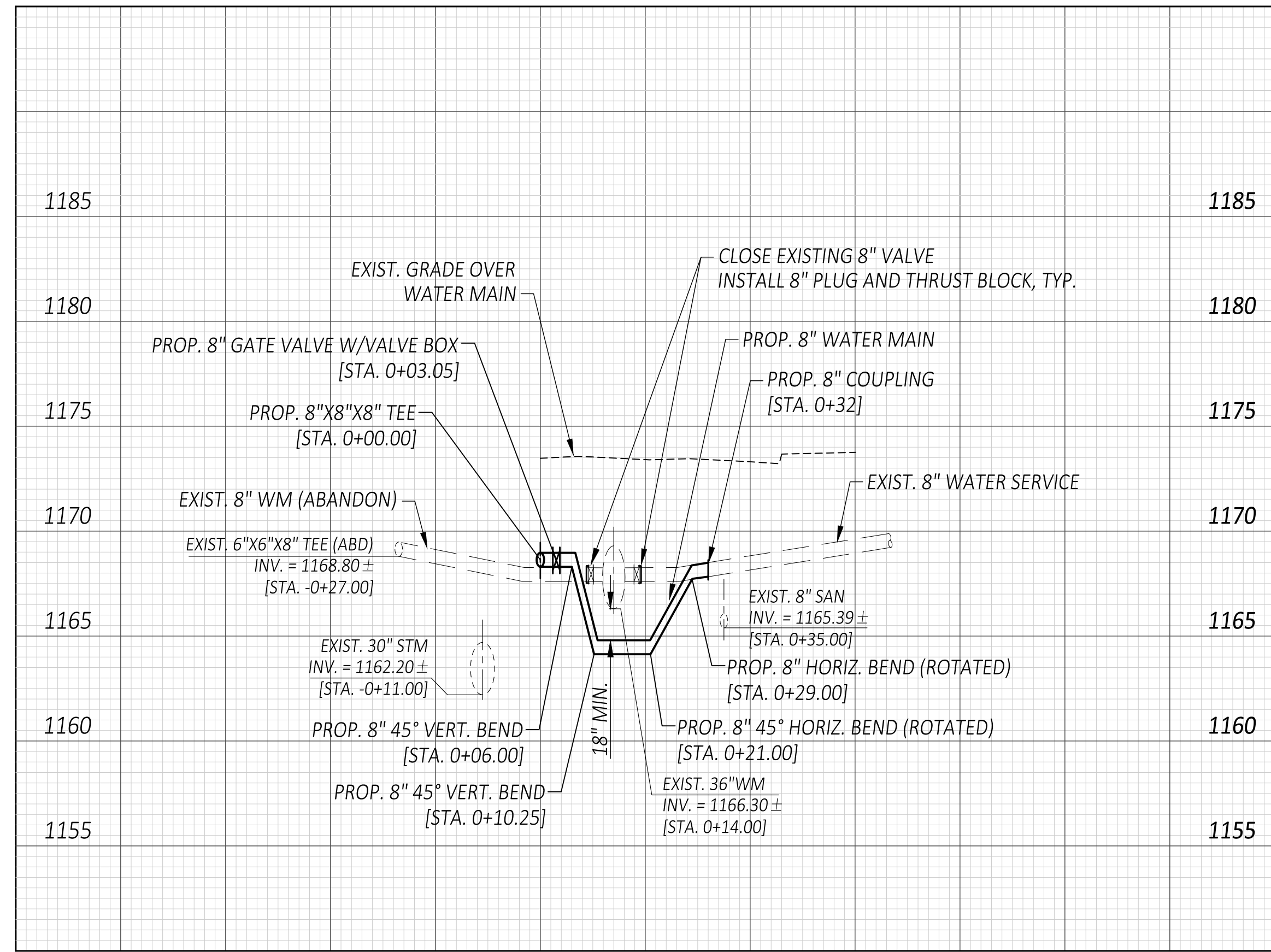
0+00 1+00 30TH STREET NW – 8" WATER SERVICE (FOR PLAN VIEW, SEE SHEET 14)
