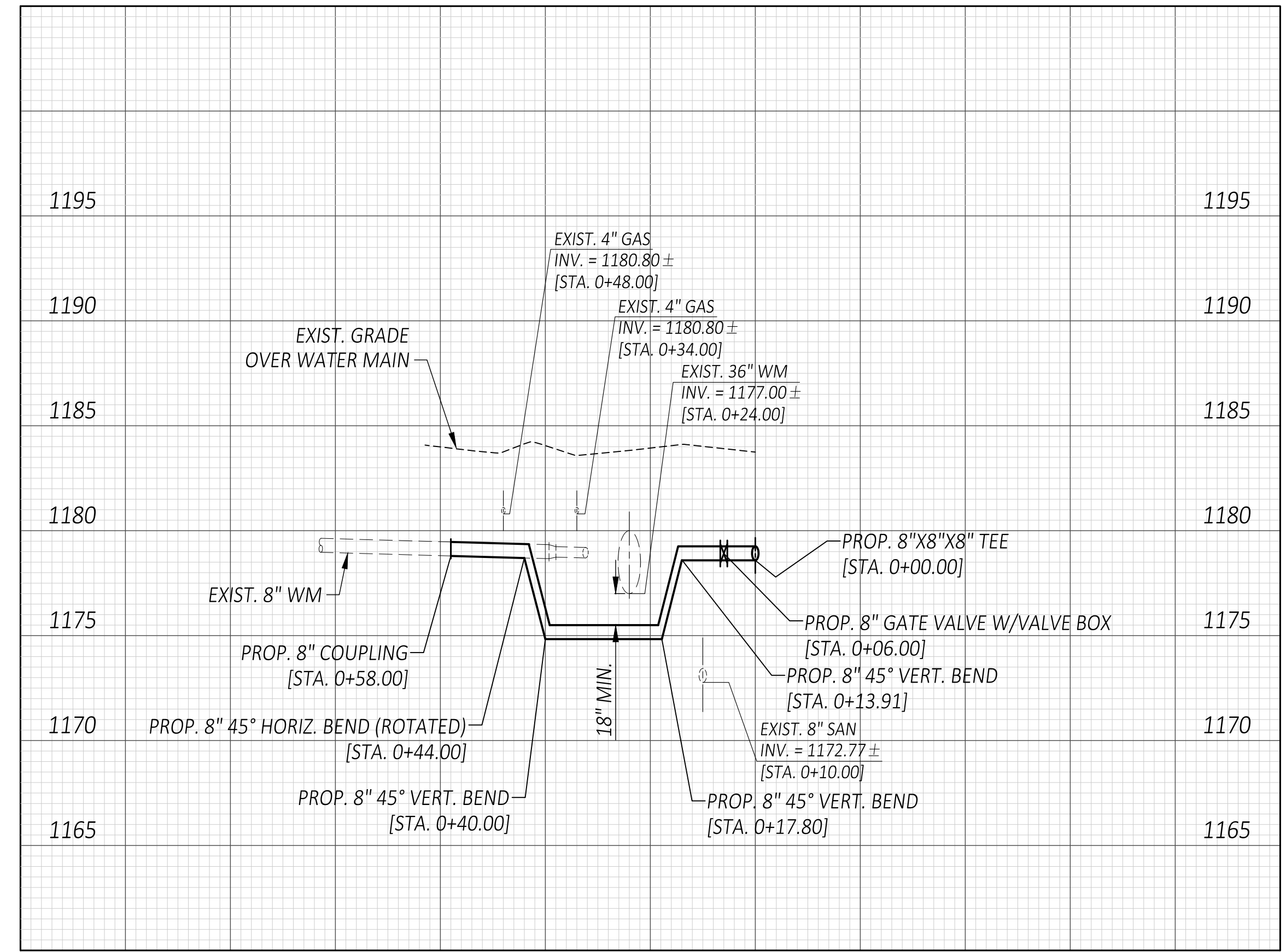
1+00 0+00 31ST STREET NW (FOR PLAN VIEW, SEE SHEET 11)
