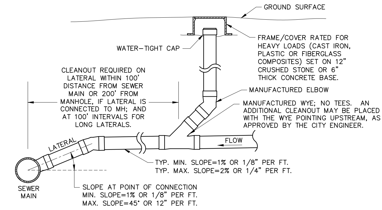
SECTION VIEW NOT TO SCALE
