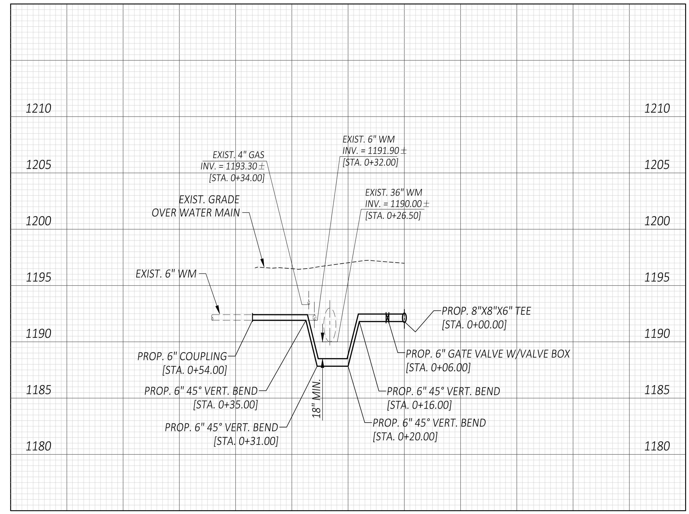
1+00 0+00 32ND STREET NW (FOR PLAN VIEW, SEE SHEET 11)
