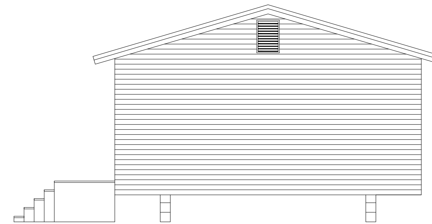
WEST SIDE ELEVATION SCALE: 1" = 4'
