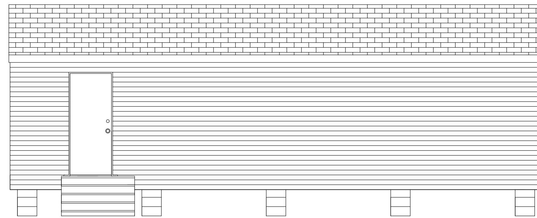
SOUTH ELEVATION SCALE: 1" = 4'
