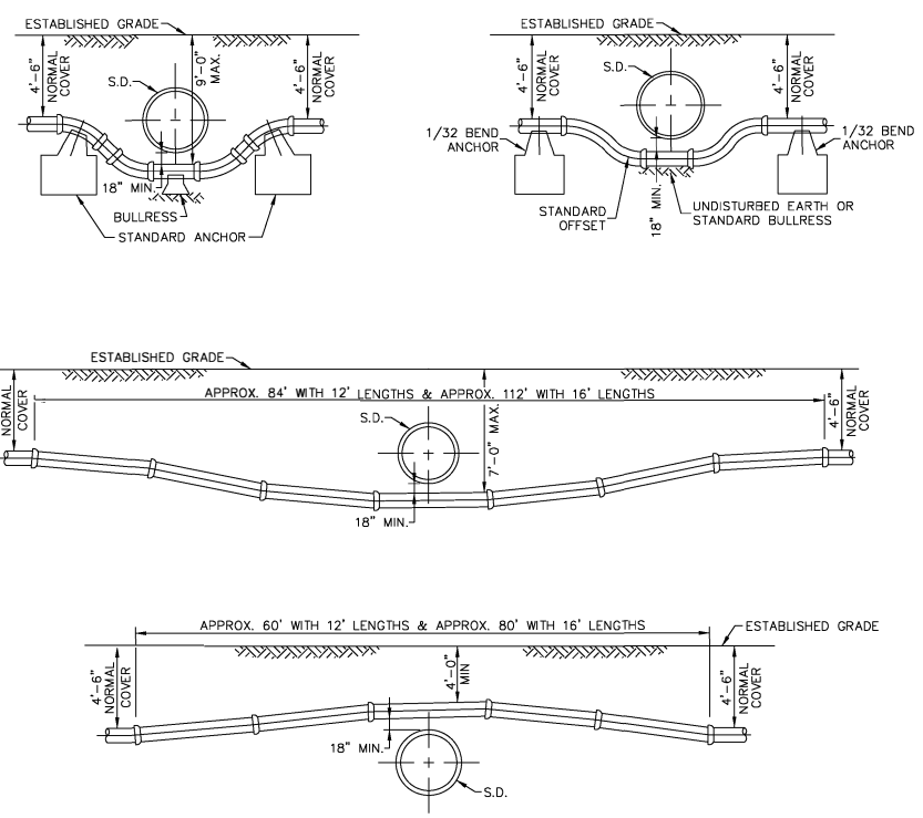
WATER MAIN CROSSING STORM DRAIN (C187)
