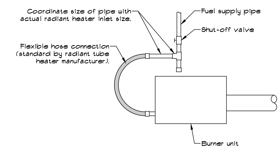
FUEL SUPPLY CONNECTION DETAIL 1" = 1'-0"
