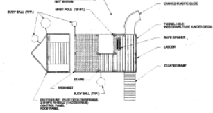
5 SHEMP BOAT - PLAN SCALE: 1/8"=1'-0"
