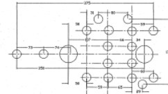
12 PIRATE SHIP - FOOTING PLAN SCALE: 1/8"=1'-0"
