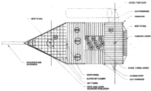
9 PIRATE SHIP - PLAN SCALE: 1/8"=1'-0"
