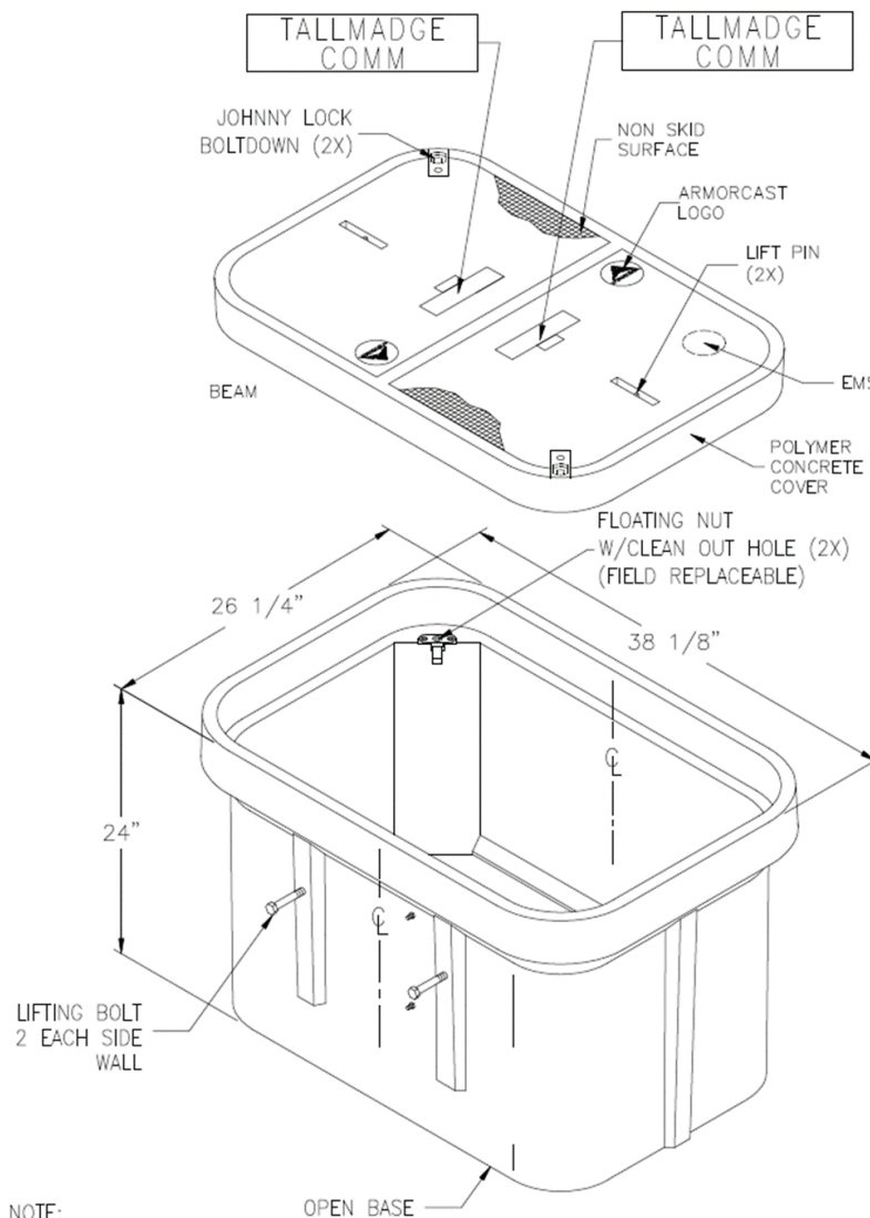
24" X 36" X 24" POLYMER CONCRETE BOX ASSEMBLY
