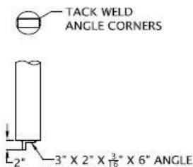
POLE BOTTOM DETAIL
