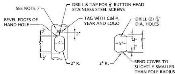
HAND HOLE DETAIL
