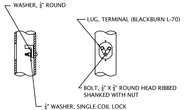
GROUNDING DETAIL
