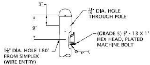
POLE TOP DETAIL
