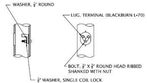
GROUNDING DETAIL
