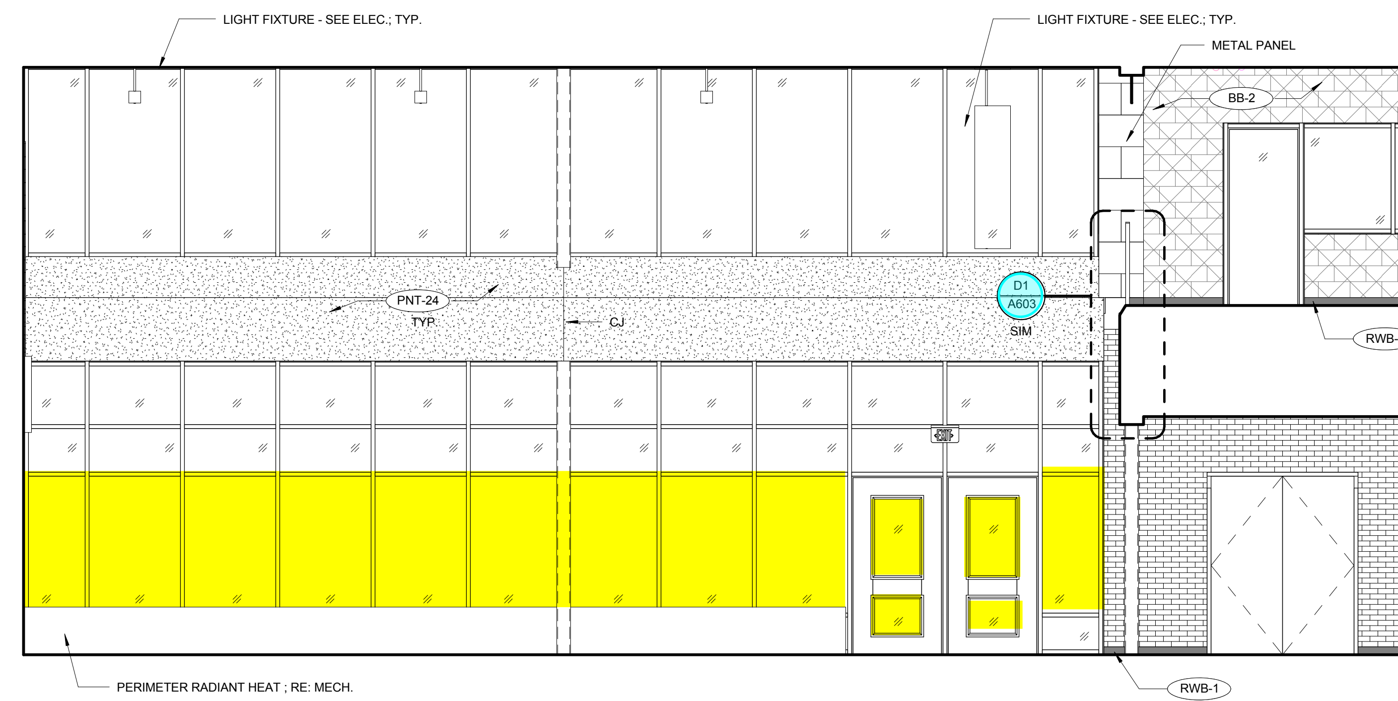
F6 A150 SOUTH 1/4" = 1'-0" REFERENCED ON A4 / A111A
