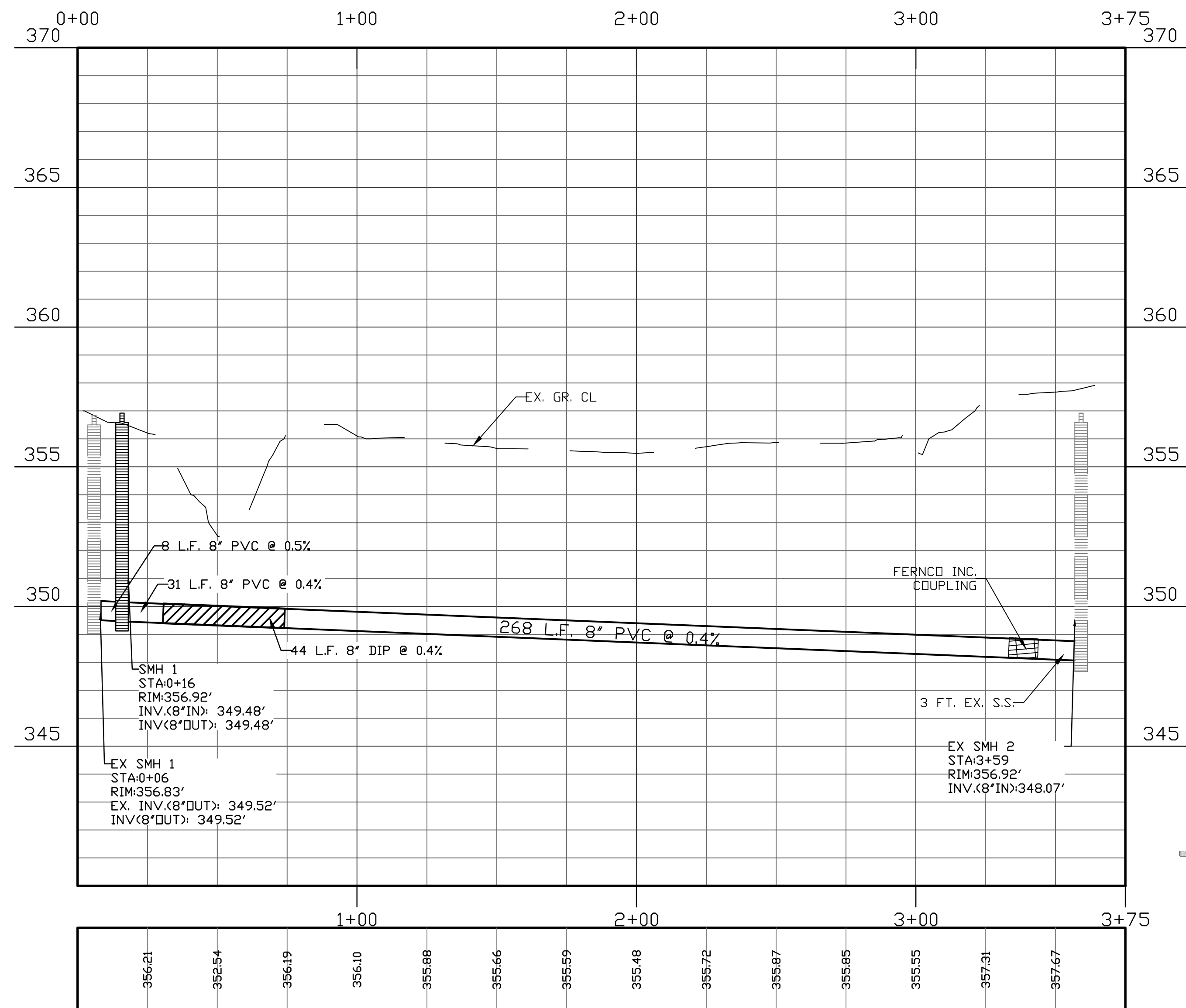
SEWER TRUNK LINE 1 ALIGNMENT PROFILE
