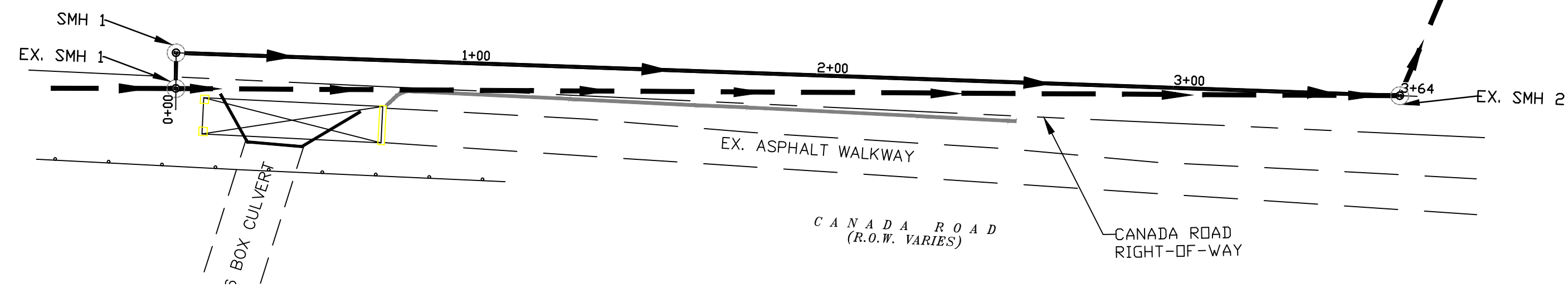
SEWER TRUNK LINE 1 ALIGNMENT PROFILE
