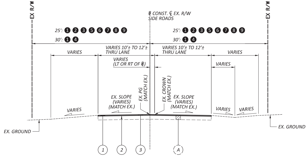
TYPICAL #1 PLANING & RESURFACING SECTION WITHOUT CURB
