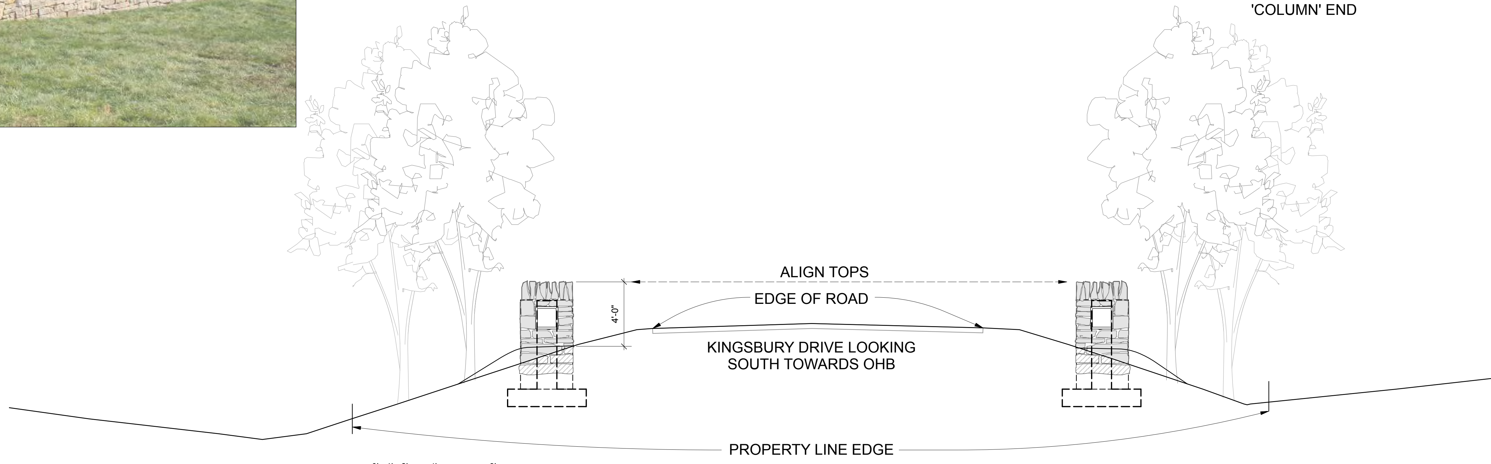
DETAIL 1: END OF WALL ELEVATION THROUGH ROAD SCALE: 1/4" = 1' - 0"
