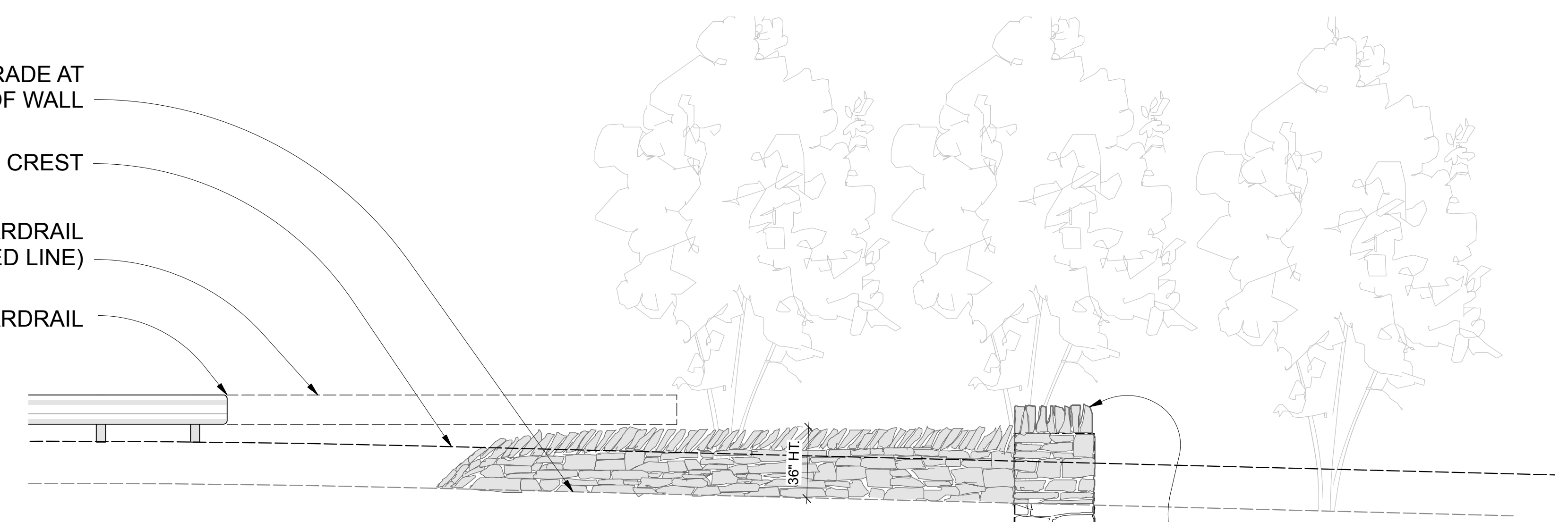
DETAIL 2: WALL SIDE ELEVATION ALONG ROAD WITH 'COLUMN' END SCALE: 1/4" = 1' - 0"
