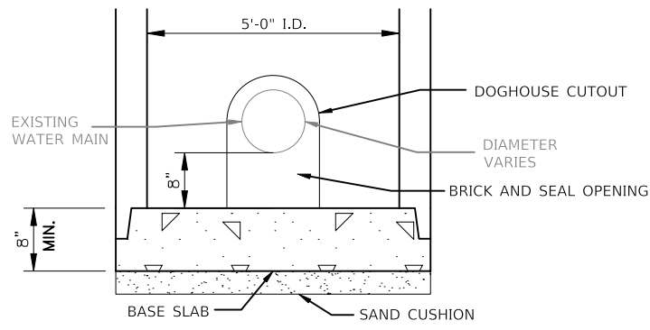
C 4 DOGHOUSE CUTOUT
