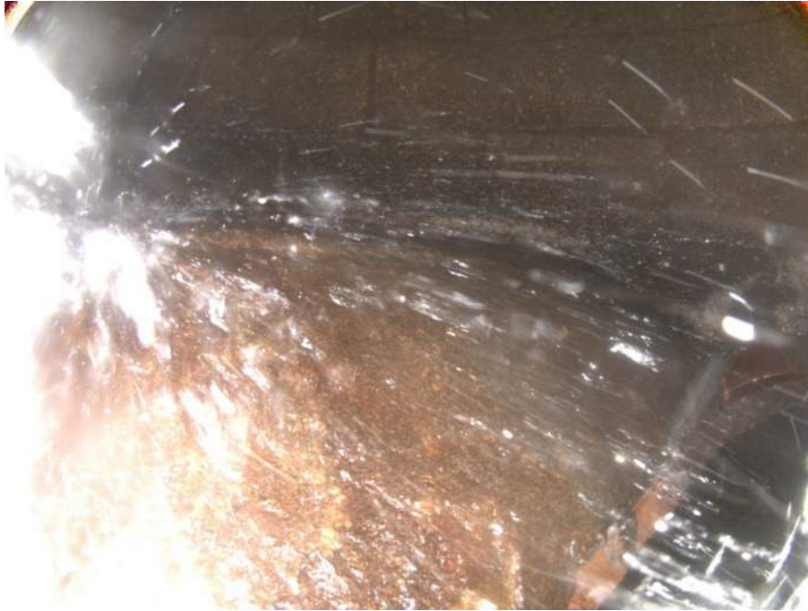
1838_4d464b94-a957-4557-a7ae-8bb14bf4d783_8215d7ef-ee63-4f71-aeed-bba2ebaa76ec_P11.jpg, 00:00:38, 8.46 Infiltration Weeper from 12 o'clock to 1 o'clock, within 8 inch
