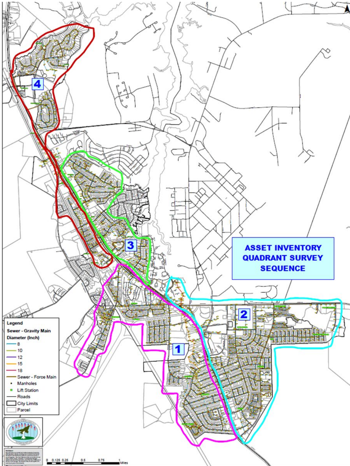
Figure 1: City Sewer Map with proposed quadrant phases.
