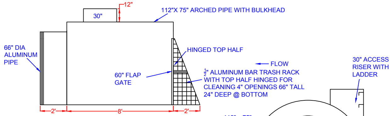
SIDE VIEW
